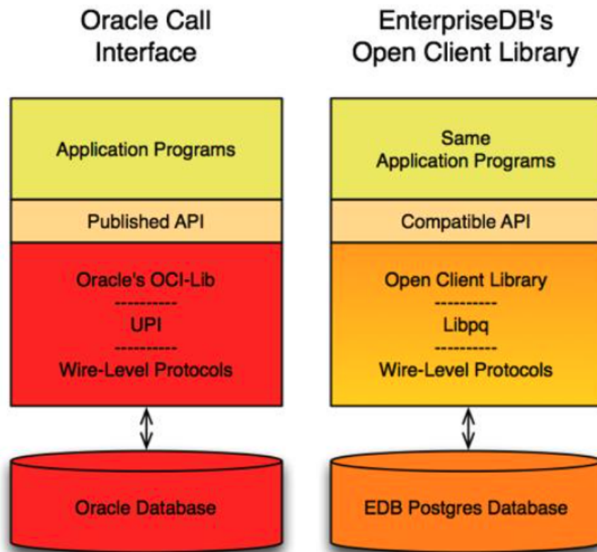
Fig. 1: The Open Client Library
