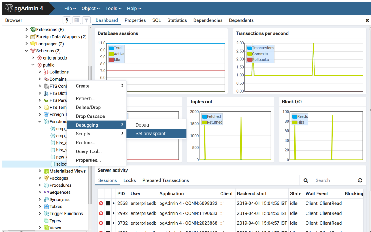
Fig. 14: Set a breakpoint by clicking in left-hand margin
