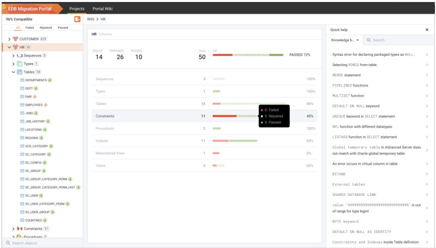
Fig. 4.7: Verifying the DDL objects.
