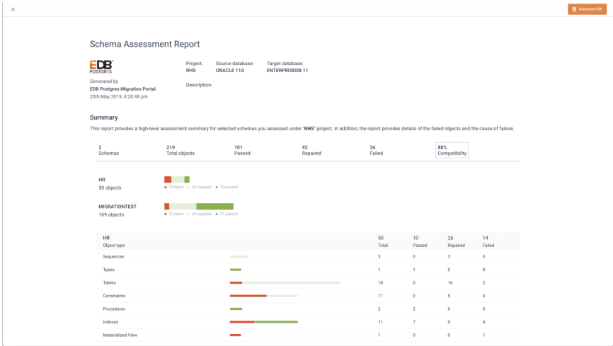
Fig. 4.12: The Schema Assessment Report.
