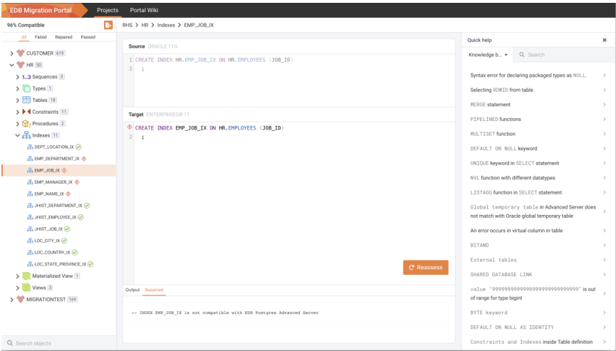
Fig. 4.8: Incompatible objects are identified.
