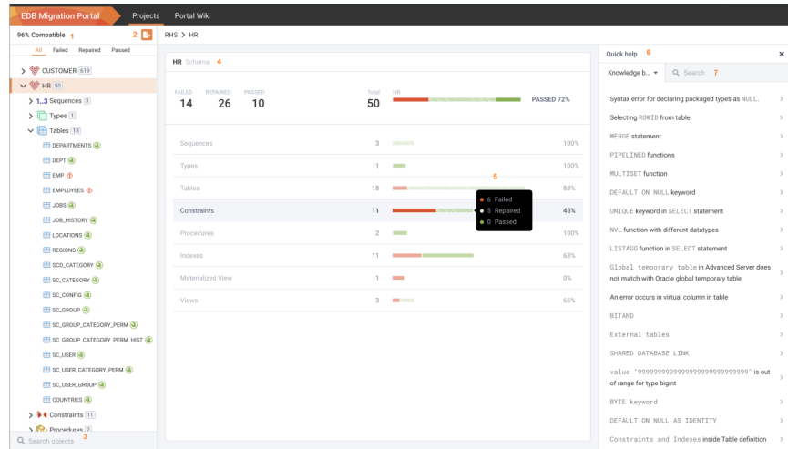
Fig. 3.4: The Migration Portal Projects Page overview.
