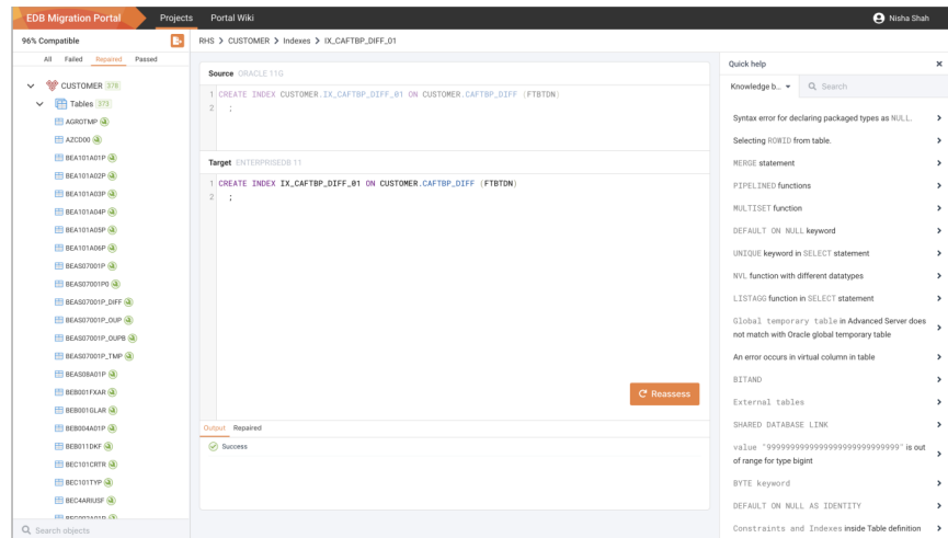
Fig. 4.10: Workaround or resolution for incompatible object.
