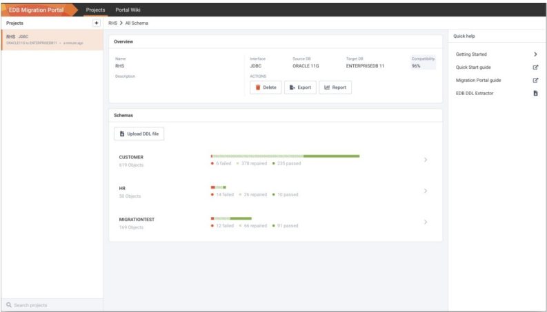
Fig. 4.6: The Schema analysis result.
