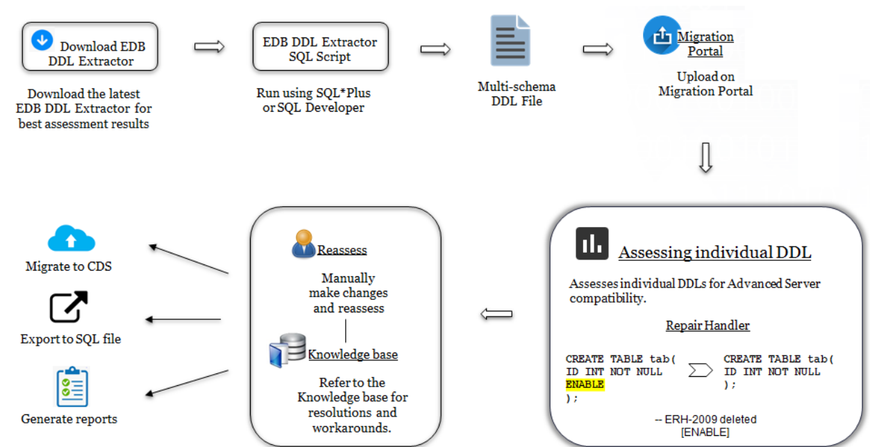
Fig. 3.1: The assessment and migration process
