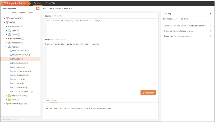
Fig. 3.5: Searching the Knowledge Base entry.
