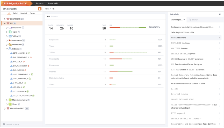
Fig. 4.9: Assessment result with errors.
