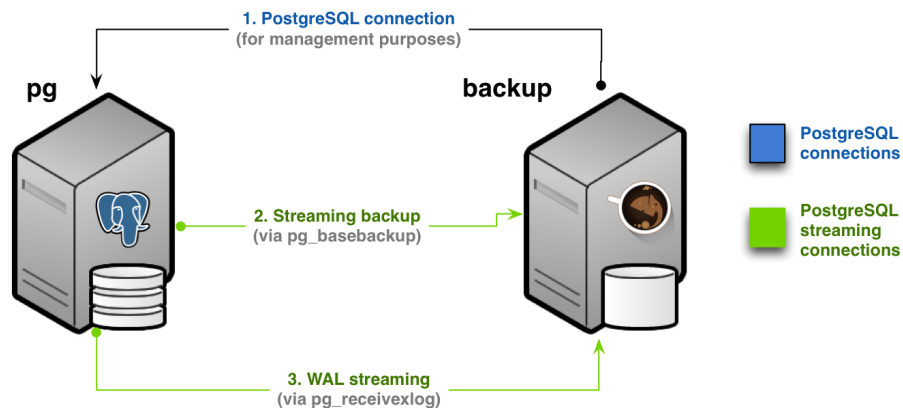
Fig. 2: Streaming-only backup (Scenario 1)
