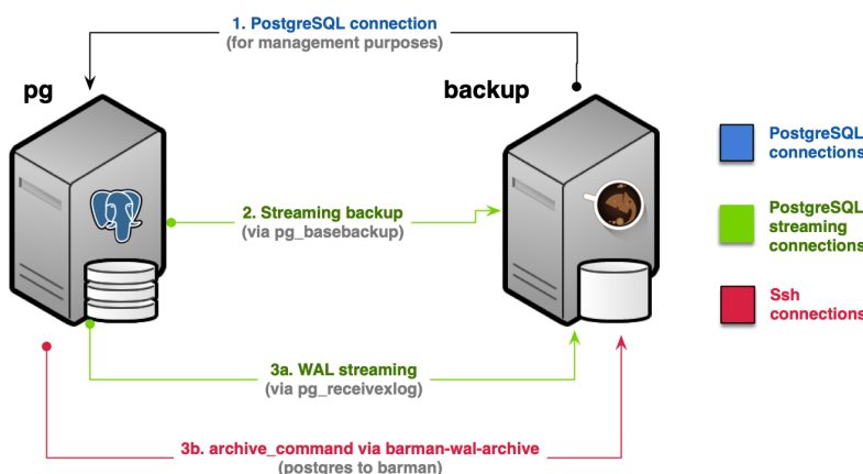
Fig. 3: Streaming backup with WAL archiving (Scenario 1b)
