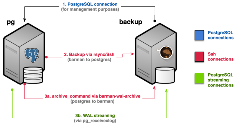
Fig. 5: Backup via rsync/SSH with WAL streaming (Scenario 2b)
