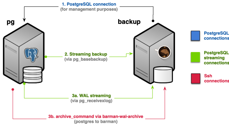
Fig. 3: Streaming backup with WAL archiving (Scenario 1b): raw-latex:label{scenario1b-design}
