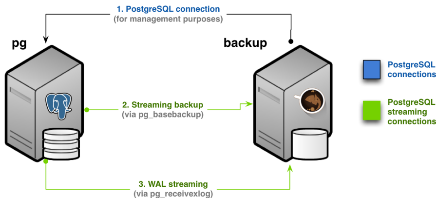
Fig. 2: Streaming-only backup (Scenario 1):raw-latex:label{scenario1-design}
