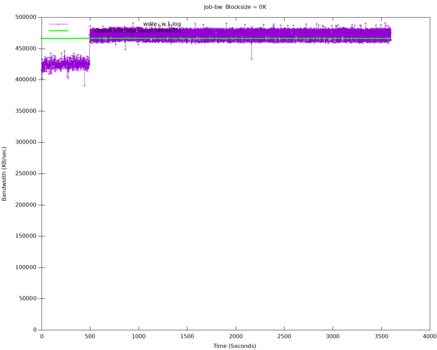
Fig. 14: Sequential writes bandwidth
