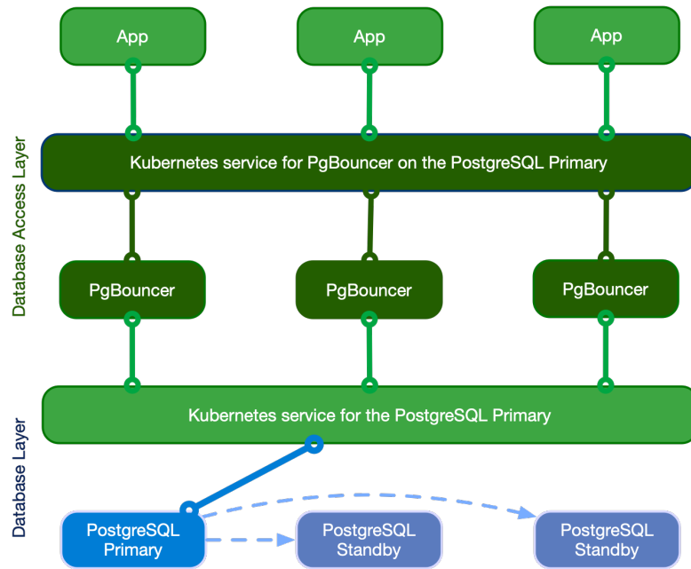
Fig. 12: Applications writing to the single primary via PgBouncer
