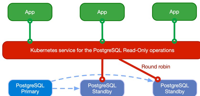
図 8: Applications reading from hot standby replicas in round robin
