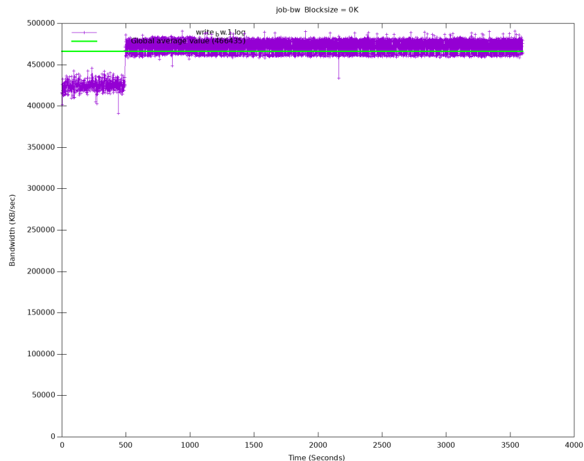
図 15: Sequential writes bandwidth
