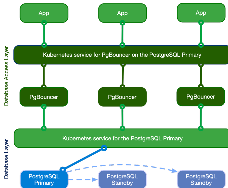
図 13: Applications writing to the single primary via PgBouncer
