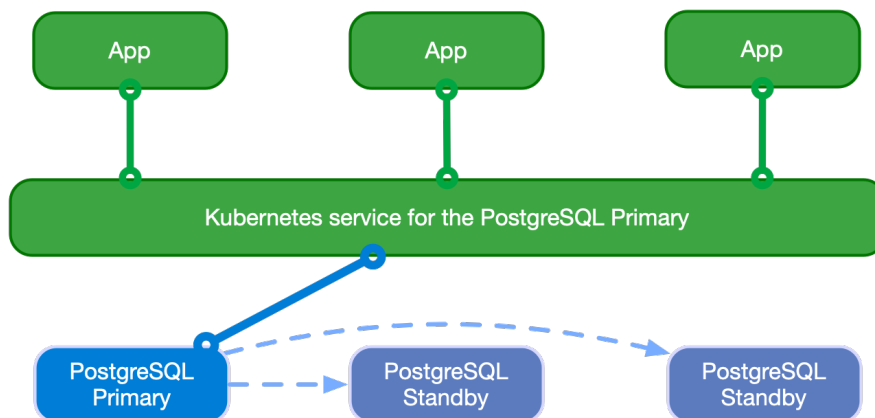
Fig. 5: Applications writing to the single primary
