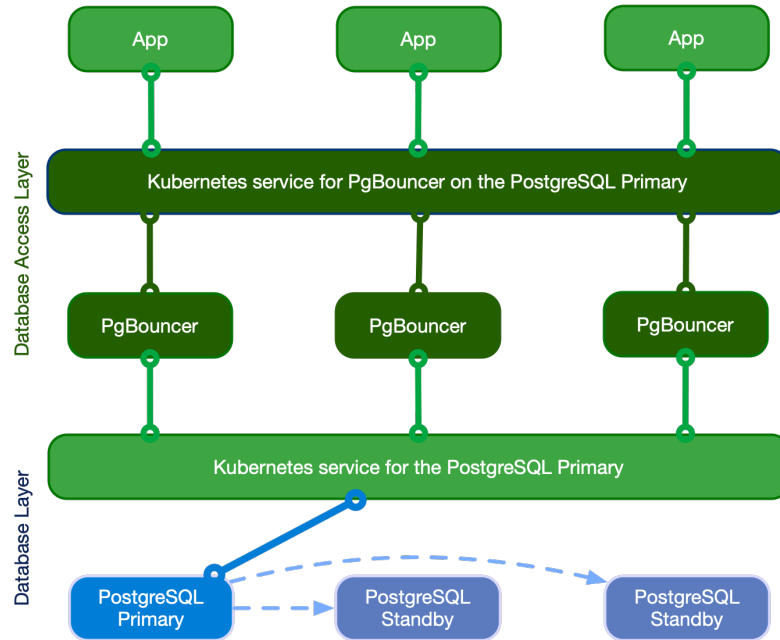
Fig. 1: Applications writing to the single primary via PgBouncer
