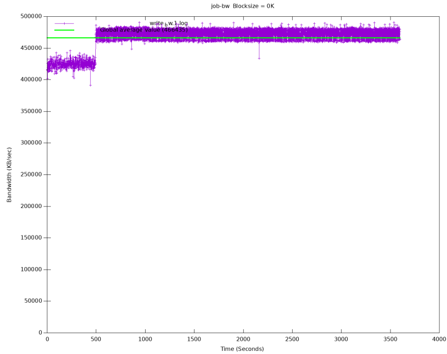
Fig. 1: Sequential writes bandwidth
