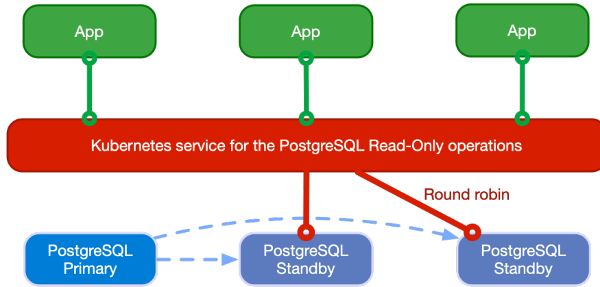
Fig. 6: Applications reading from hot standby replicas in round robin
