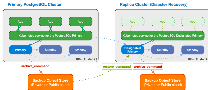
Fig. 1: An example of multi-cluster deployment with a primary and a replica cluster
