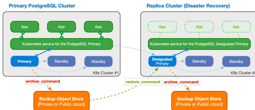
Fig. 7: An example of multi-cluster deployment with a primary and a replica cluster
