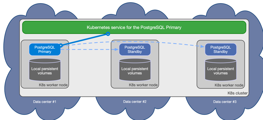
Fig. 4: Bird-eye view of the recommended shared nothing architecture for PostgreSQL in Kubernetes
