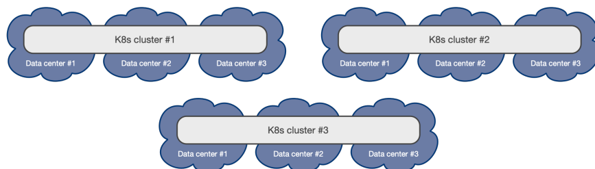
Fig. 2: Example of a multiple Kubernetes cluster architecture distributed over 3 regions each with 3 independent data centers
