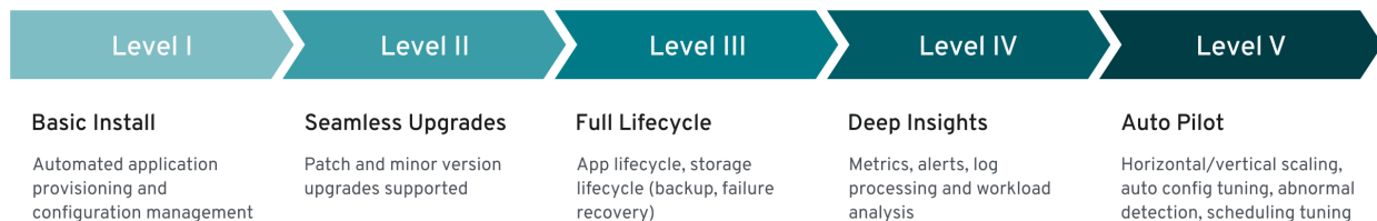
Fig. 11: Operator Capability Levels
