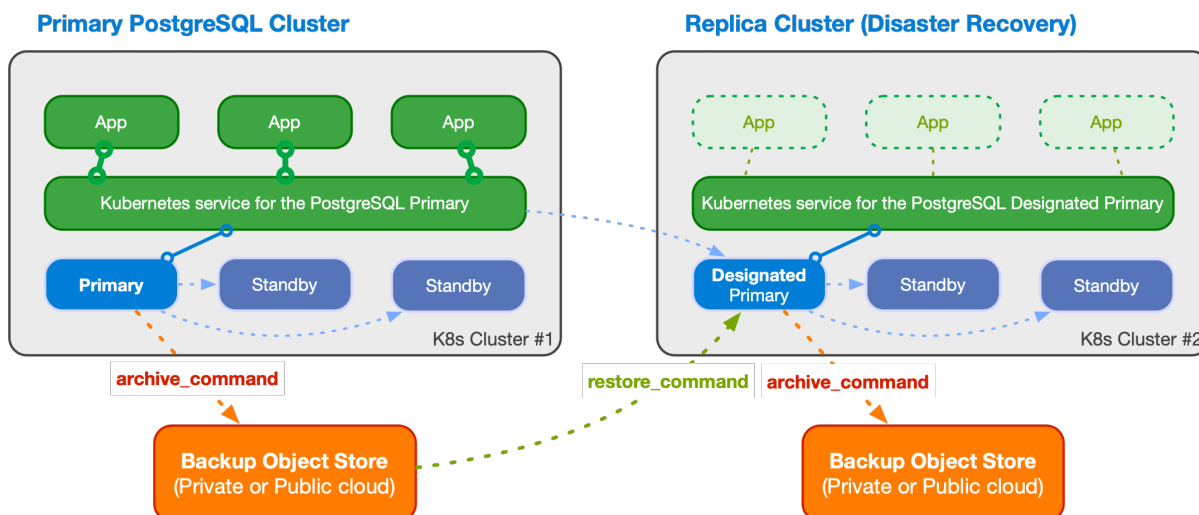
図 6: An example of multi-cluster deployment with a primary and a replica cluster
