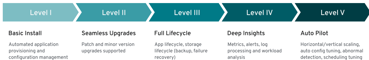
図 13: Operator Capability Levels
