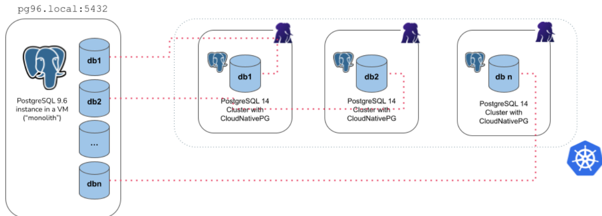
図 9: Example of microservice import type
