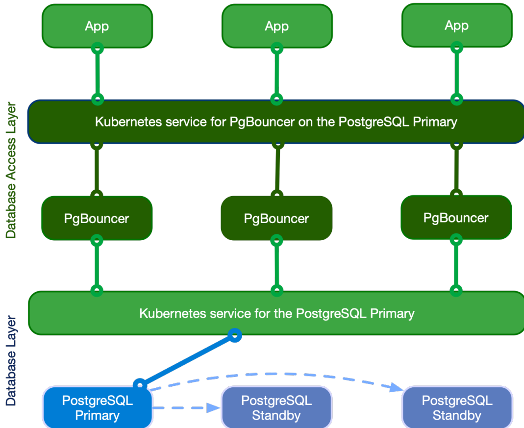
図 11: Applications writing to the single primary via PgBouncer
