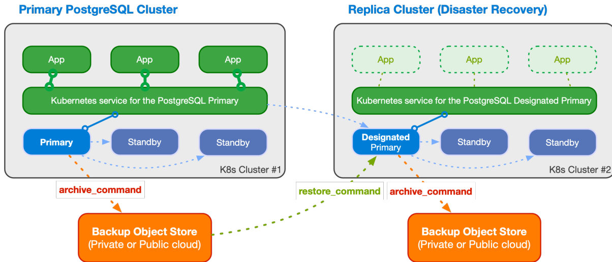
図 12: An example of multi-cluster deployment with a primary and a replica cluster
