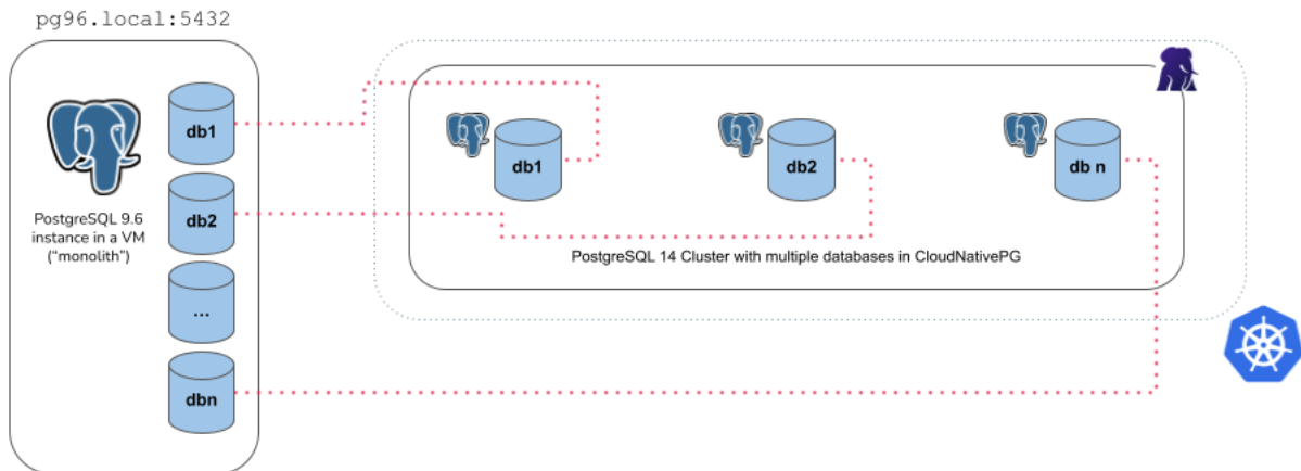
図 10: Example of monolith import type
