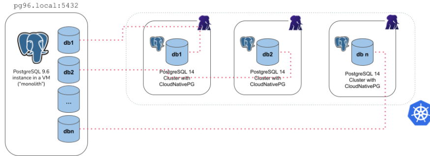
Fig. 1: Example of microservice import type
