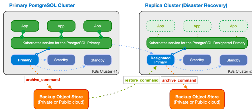
Fig. 4: An example of multi-cluster deployment with a primary and a replica cluster
