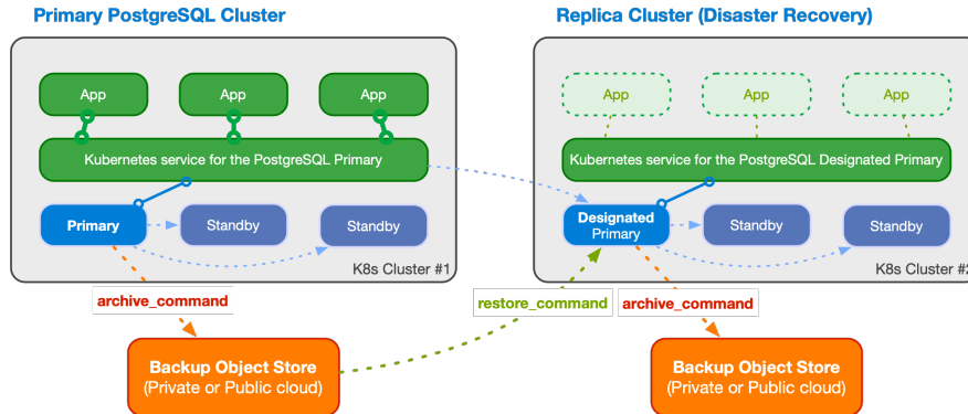
Fig. 10: An example of multi-cluster deployment with a primary and a replica cluster
