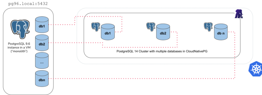
Fig. 2: Example of monolith import type
