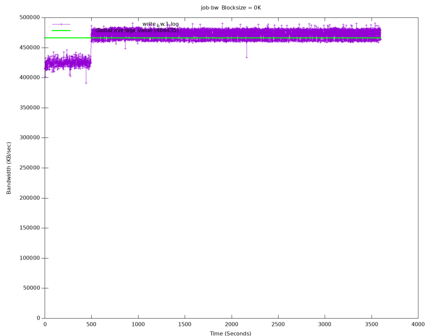
Fig. 6: Sequential writes bandwidth
