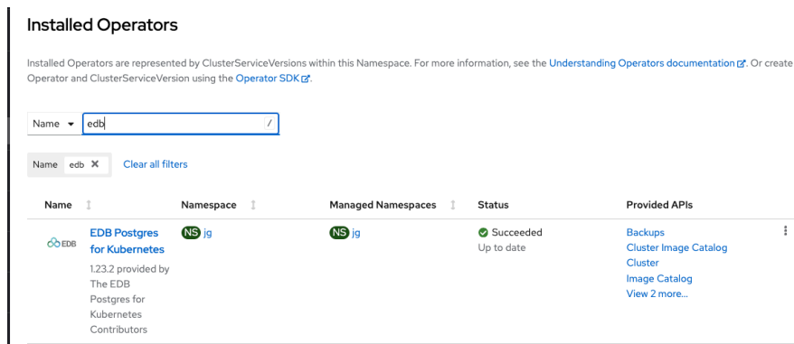
Fig. 7: Multi namespace installation displayed in the web console
