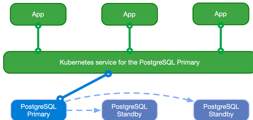
Fig. 5: Applications writing to the single primary
