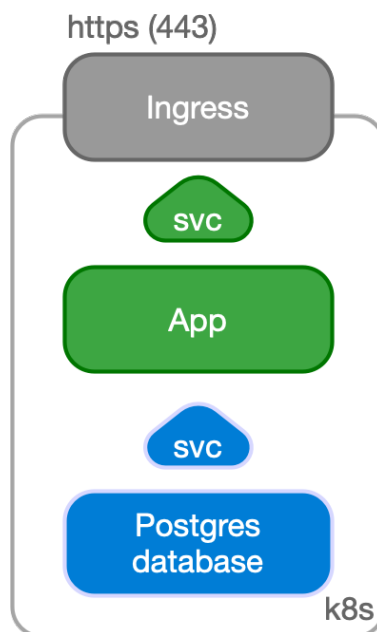
Fig. 8: Application and Database inside Kubernetes
