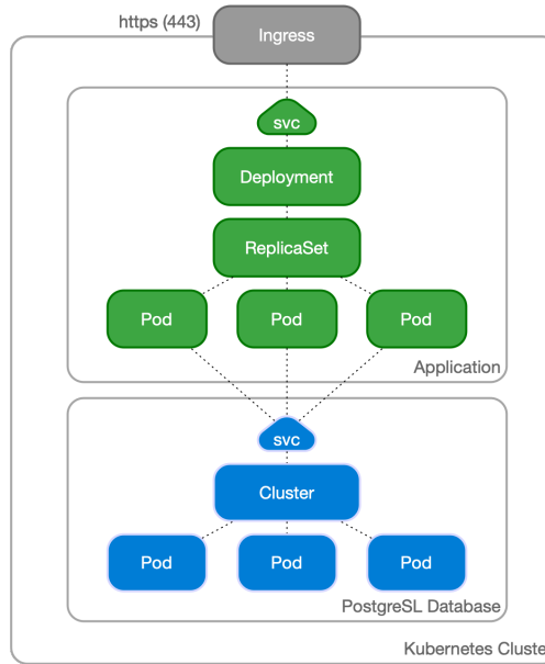
Fig. 9: Close-up view of application and database inside Kubernetes
