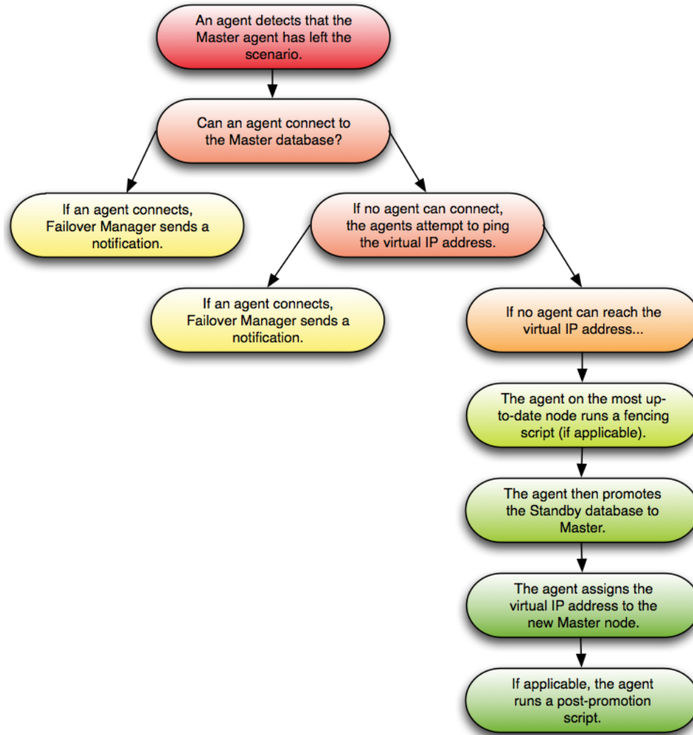
Fig. 3: Confirming the failure of the Master Agent.
