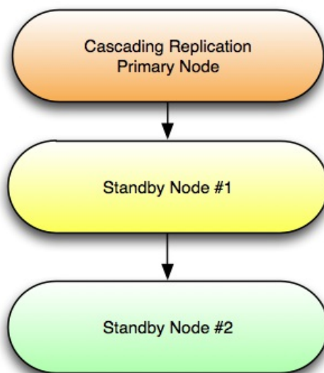
Cascading replication.
