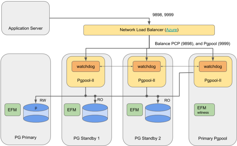
Architecture diagram for EFM and Pgpool integration using Azure Load Balancer
