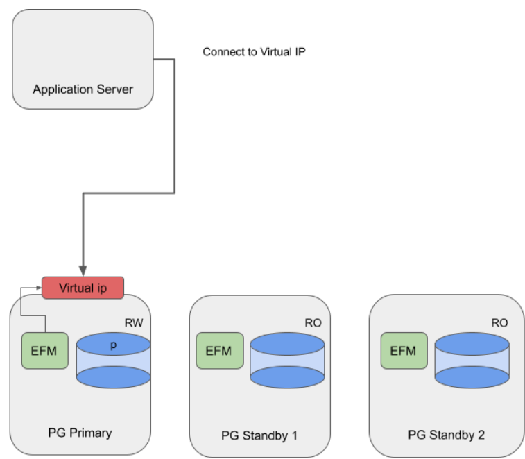
Fig. 2: Failover Manager with VIP
