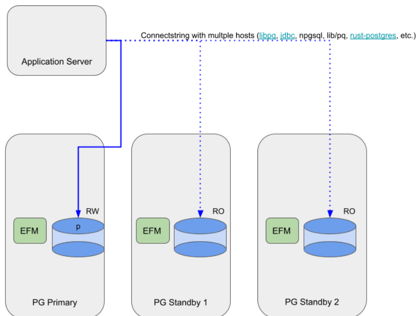
Fig. 3: Failover Manager traffic routing diagram for client connect failover
