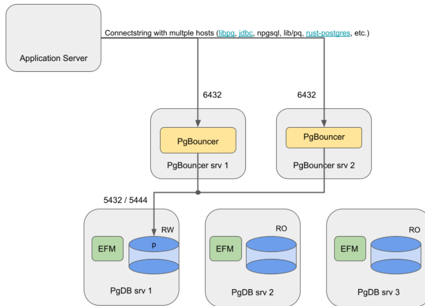
Fig. 4: Failover Manager using pgBouncer on-premises architecture diagram
