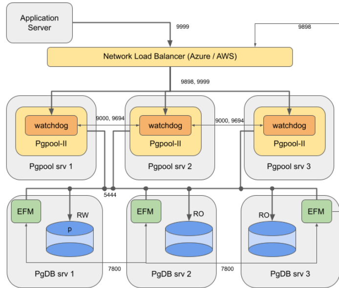
Fig. 7: Failover Manager with Pgpool in cloud
