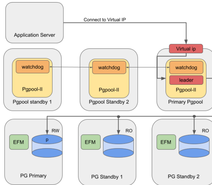
Fig. 6: Failover Manager with Pgpool on-premises
