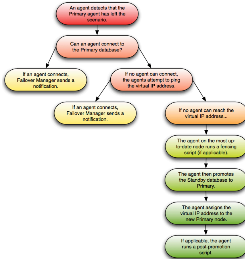
Fig. 5: Confirming the failure of the primary agent.
