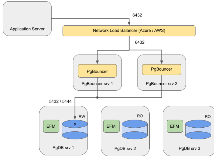
Fig. 5: Failover Manager with PgBouncer cloud architecture diagram
