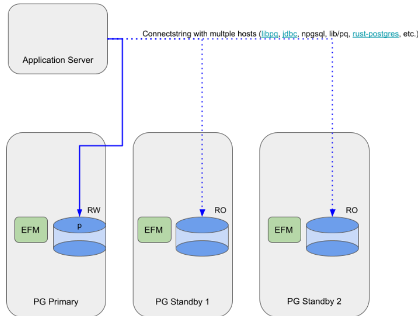
図 3: Failover Manager traffic routing diagram for client connect failover
