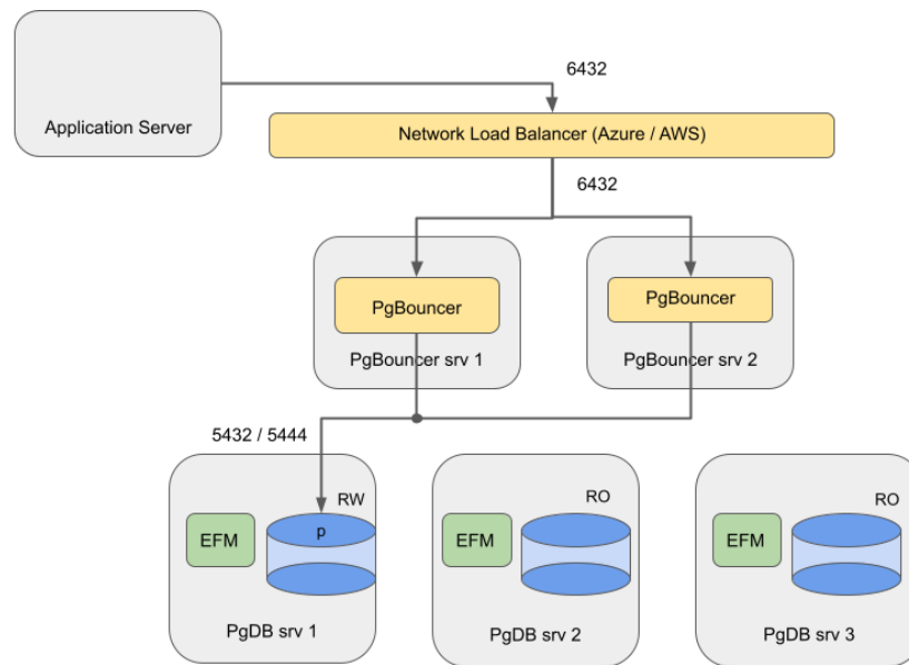
図 3: Failover Manager with PgBouncer cloud architecture diagram
