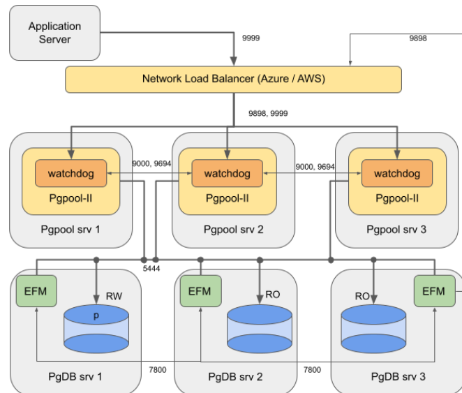
図 5: Failover Manager with Pgpool in cloud
