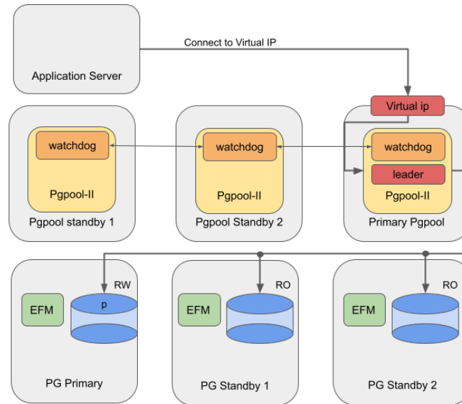
図 4: Failover Manager with Pgpool on-premises
