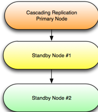
図 1: Cascading replication.
