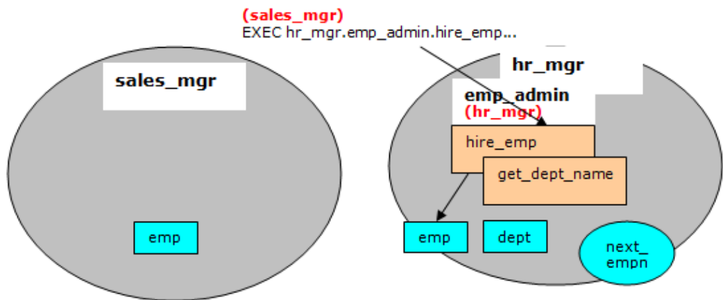
Fig. 3: Definer's Rights Package
