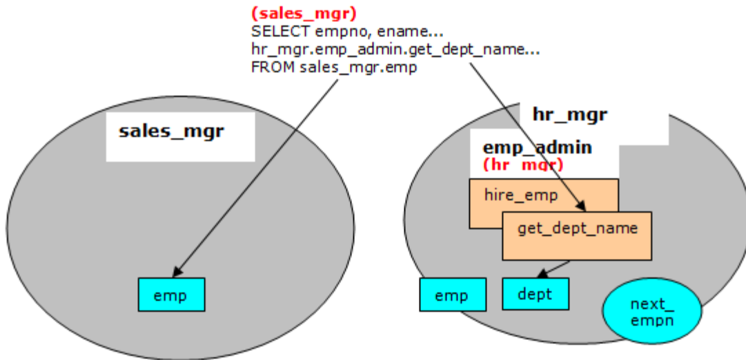
Fig. 2: Definer's Rights Package
