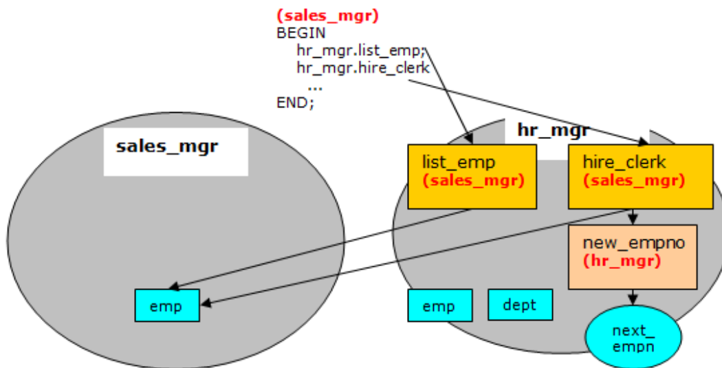
Fig. 1: Invokers Rights Programs
