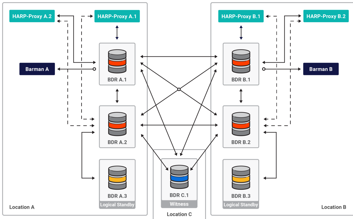
Fig. 4: Always On Platinum architecture
