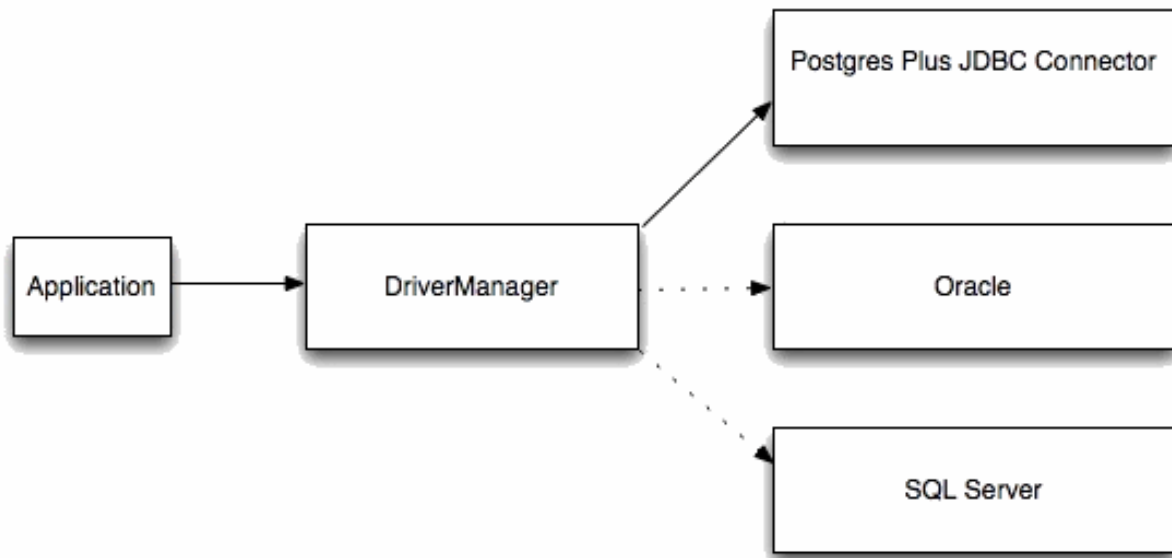
Fig. 3: DriverManager/Drivers
