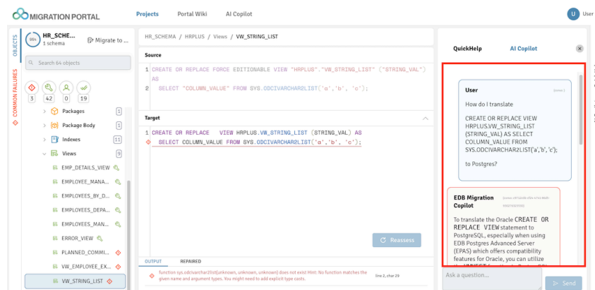
図 4: Suggestions provided by AI Copilot
