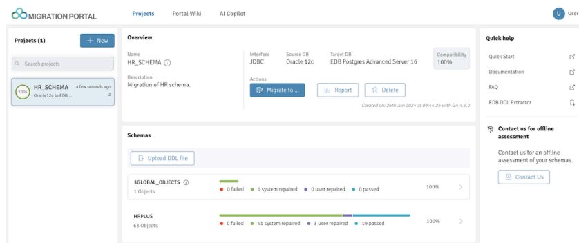
図 2: The Migration Portal home page.
