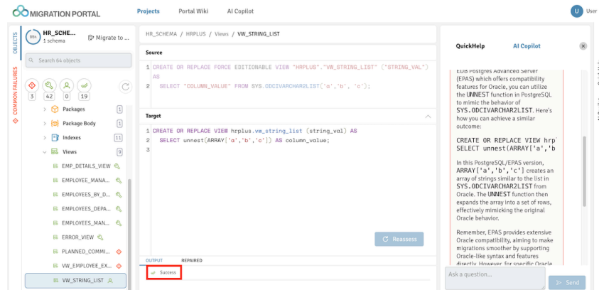
図 5: Workaround or resolution for incompatible objects
