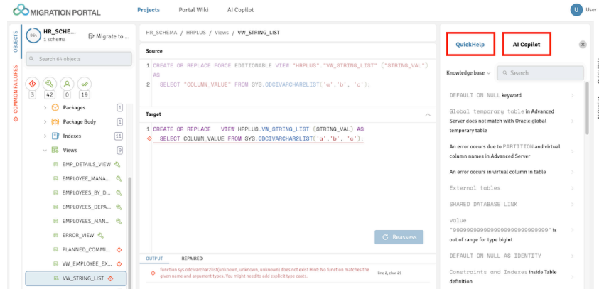
図 3: Incompatible objects are identified
