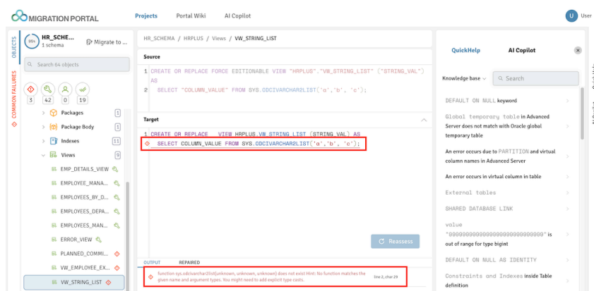
図 2: Incompatible objects are identified
