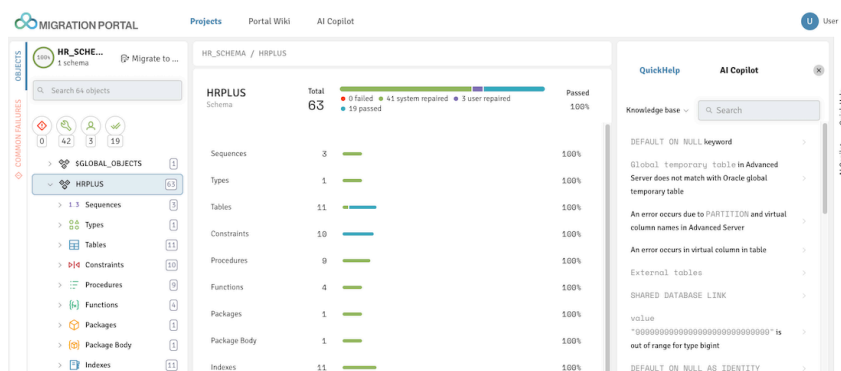
図 3: The Migration Portal Projects Page overview.
