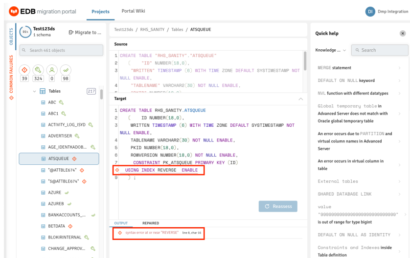
図 2: Incompatible objects are identified
