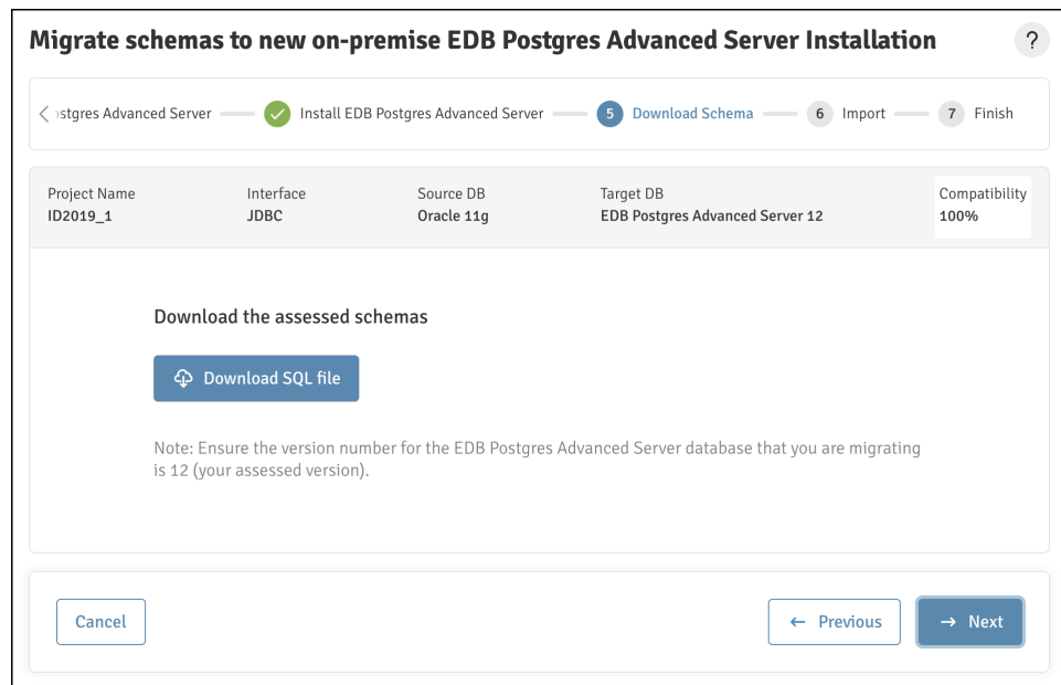
Fig. 38: Downloading the assessed schemas
