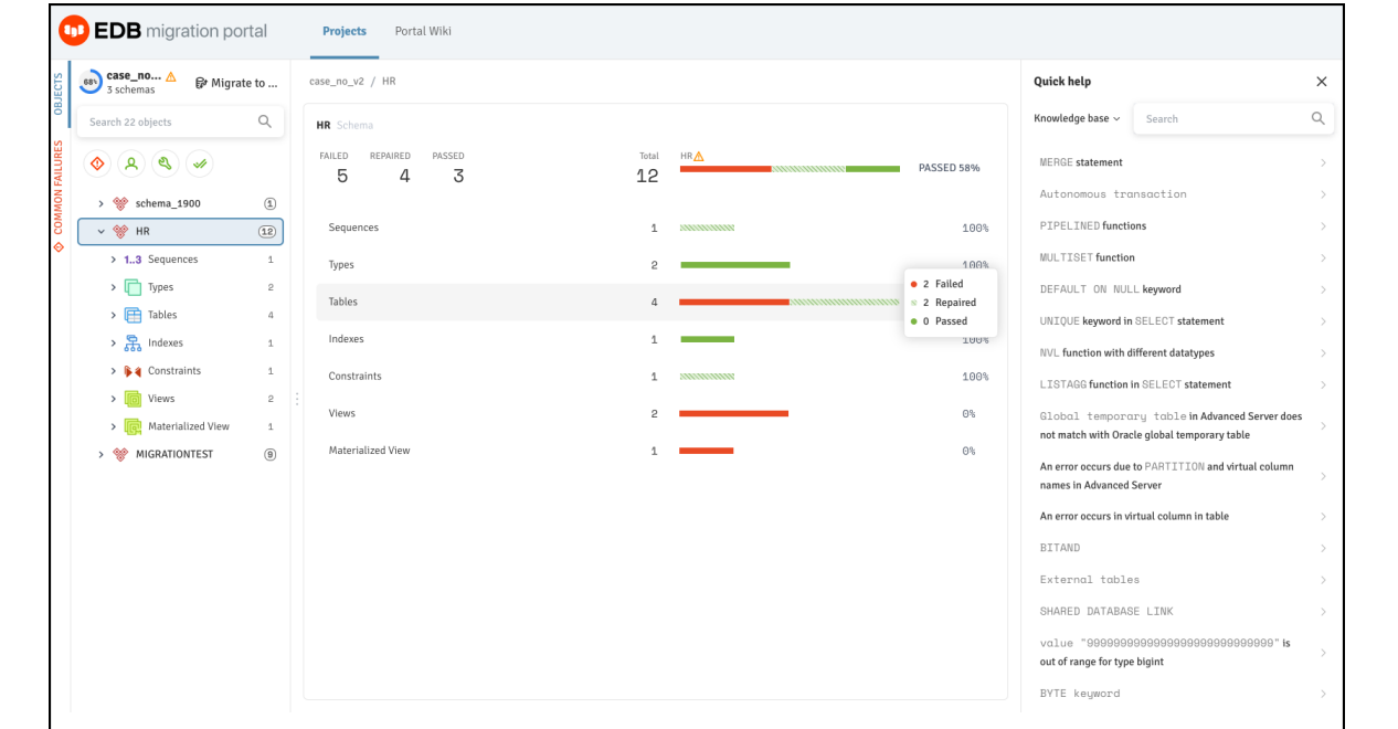
Fig. 9: Assessment result with errors.
