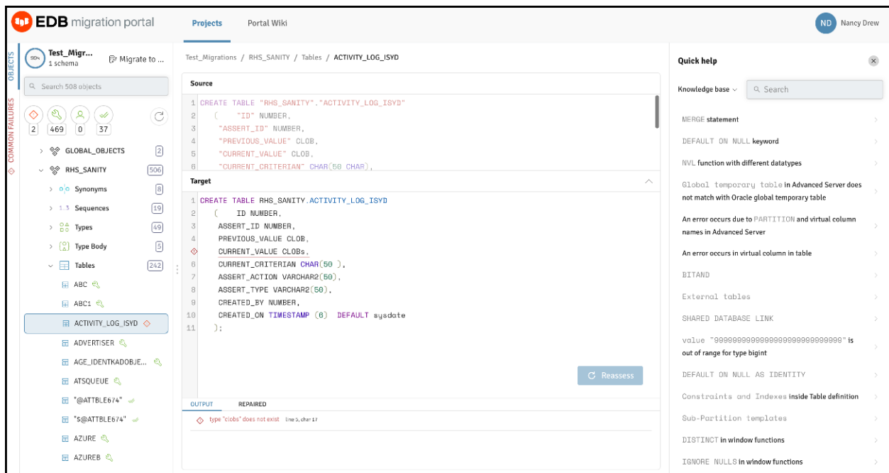
Fig. 8: Incompatible objects are identified.
