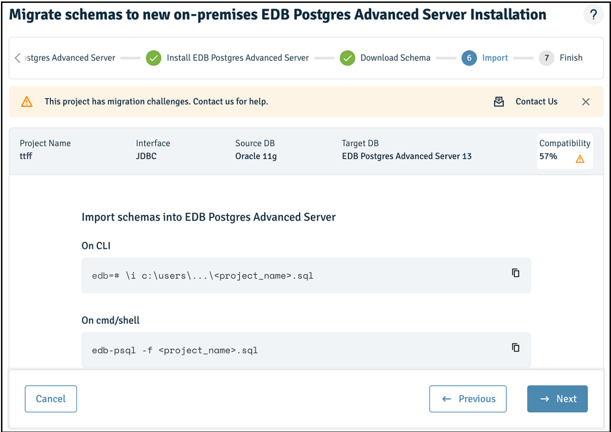
Fig. 33: Importing schemas into EDB Postgres Advanced Server
