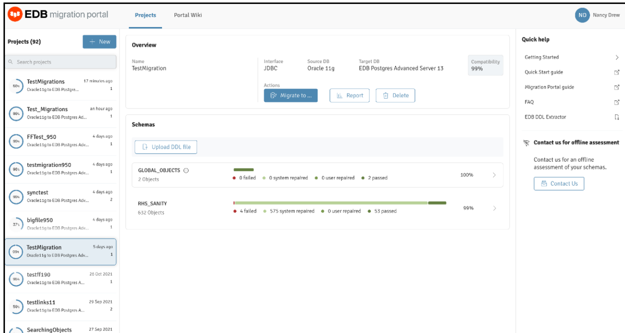
Fig. 6: The Schema analysis result.
