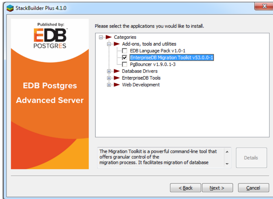
Fig. 2: The Stack Builder application selection window.
