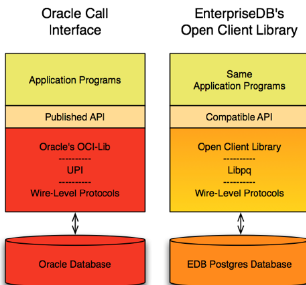
Fig. 1: Comparison with Oracle Call Interface
