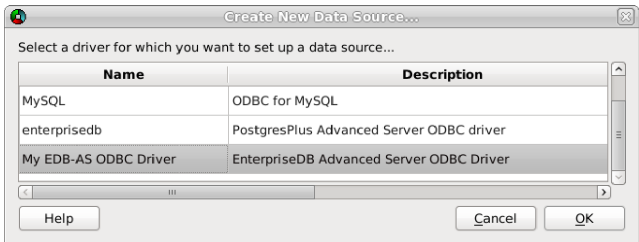
Fig. 12: Select a driver for the named data source
