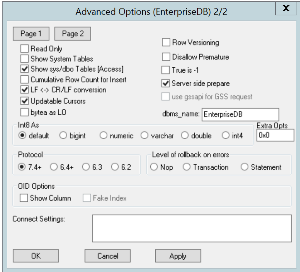
Fig. 5: Page 2 of the Advanced Options dialog
