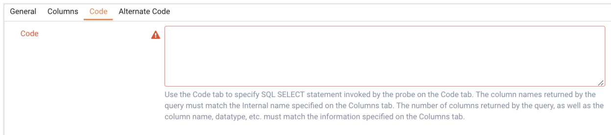
Fig. 24: The Code tab of the Custom Probes dialog
