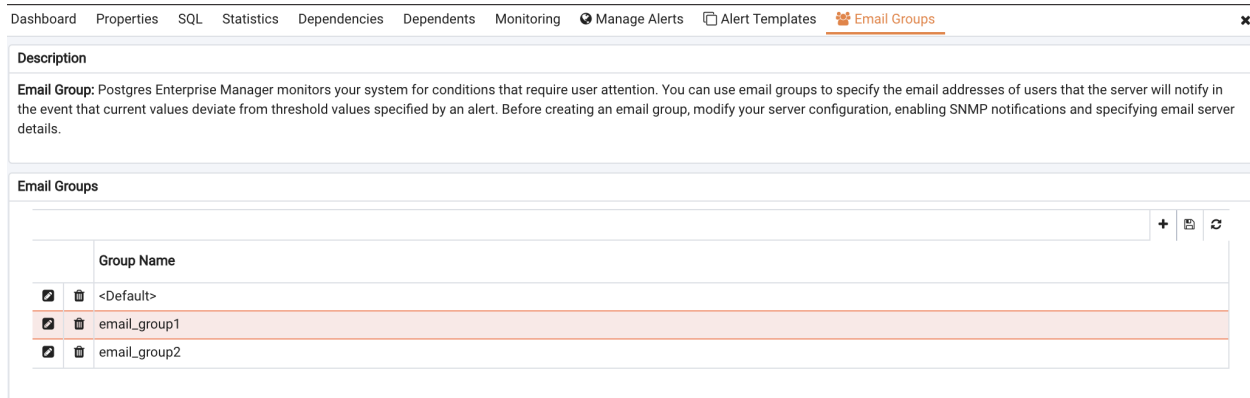
Fig. 45: The Email Groups tab
