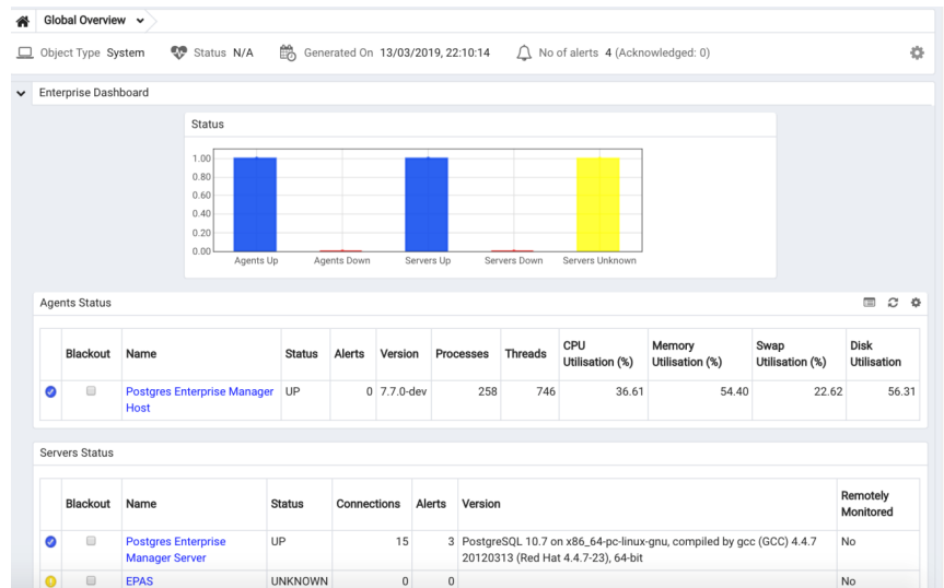
Fig. 10: The Global Overview dashboard
