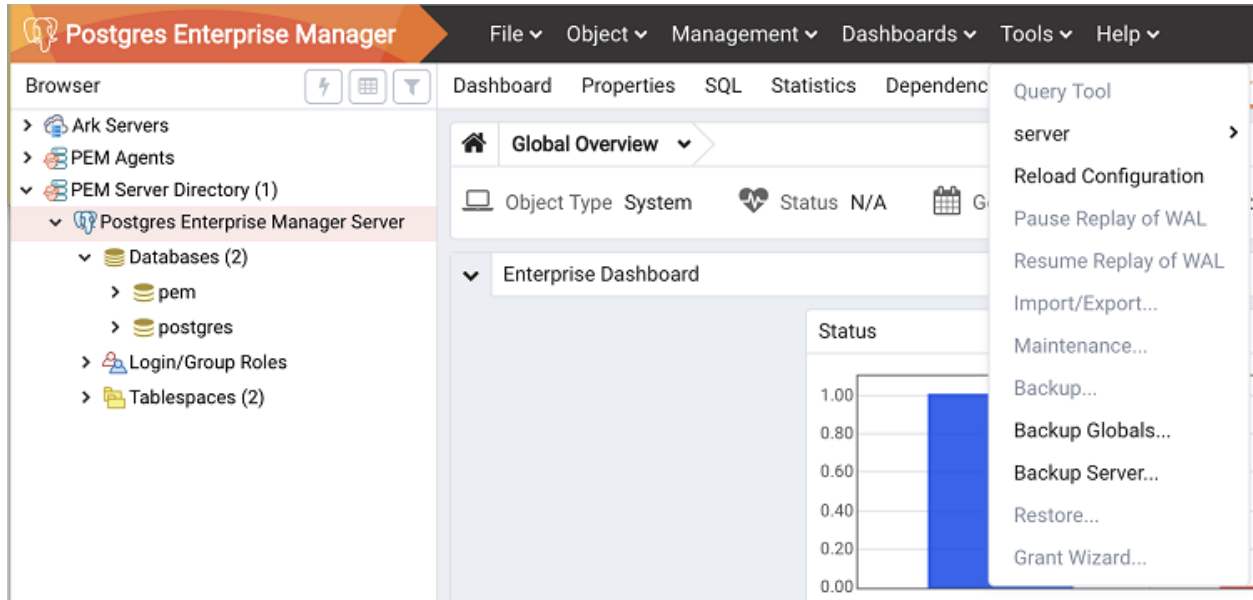
Fig. 8: The Tools menu
