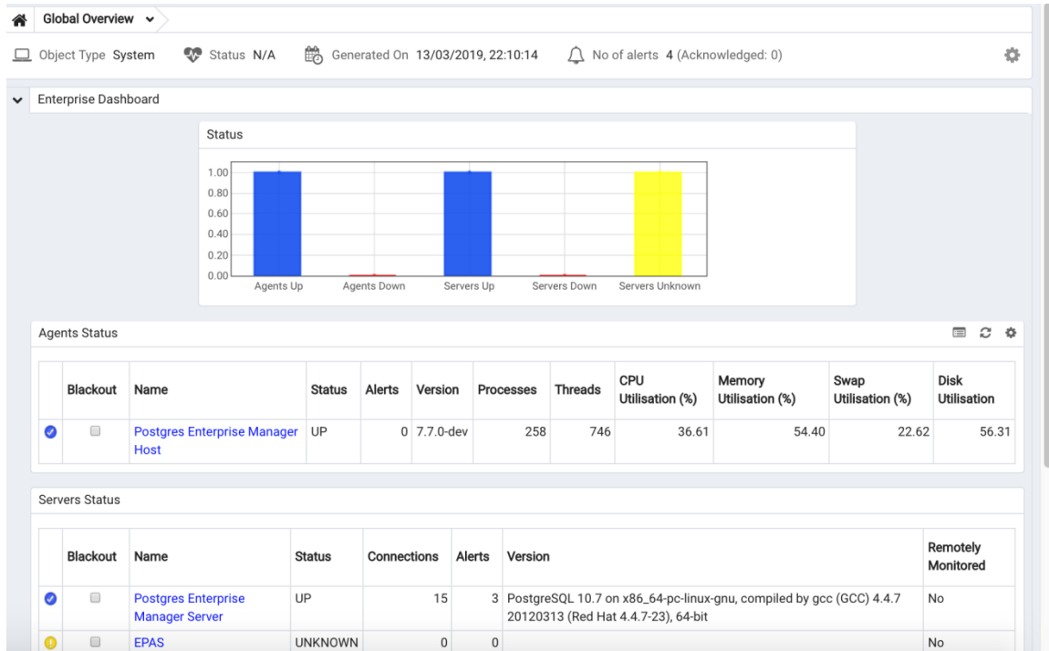
Fig. 3: The Global Overview dashboard, displayed in the client
