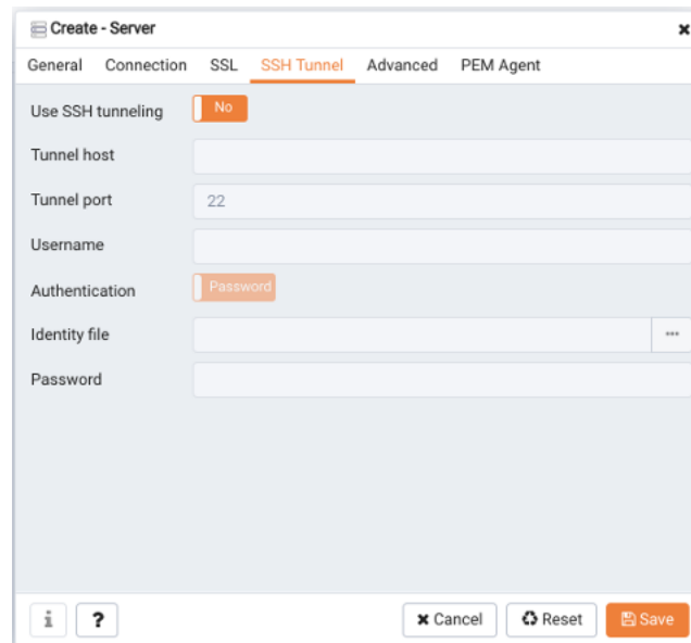
Fig. 5: The SSH Tunnel tab of the Create – Server dialog
