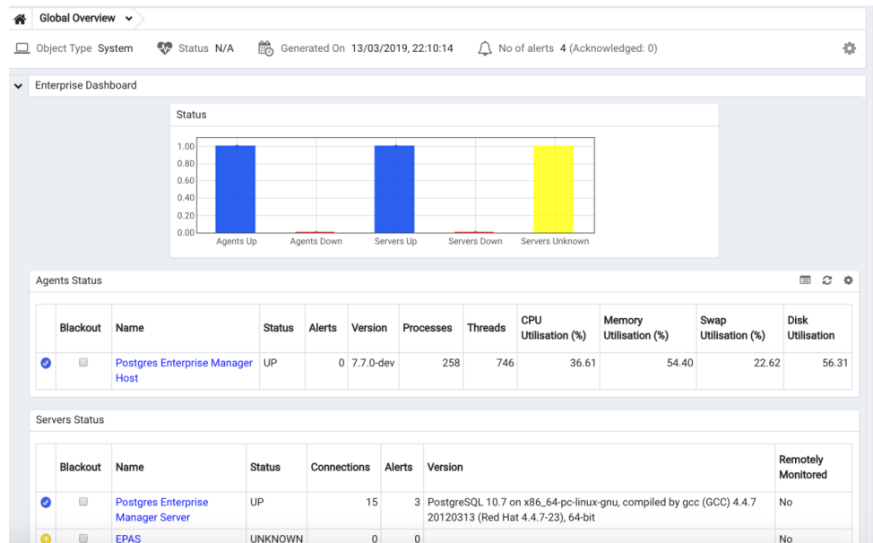
Fig. 9: The registered server
