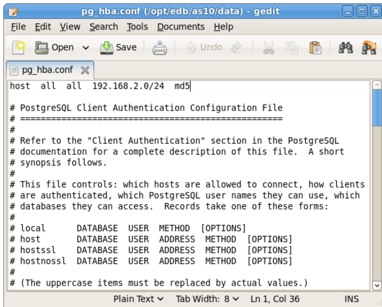
図 5 PEM entries in the pg_hba.conf file
