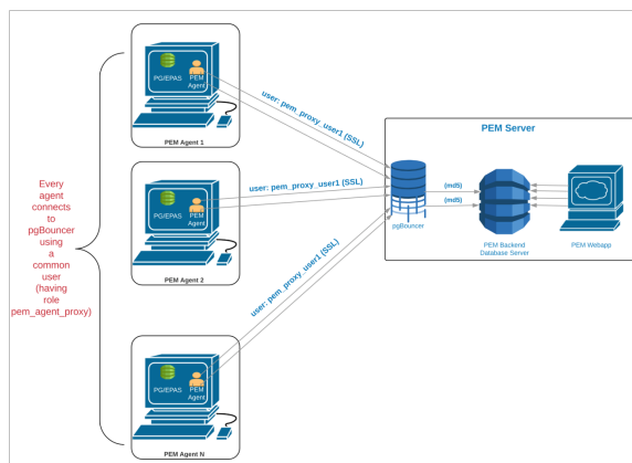
図 2 Connecting to pgBouncer.
