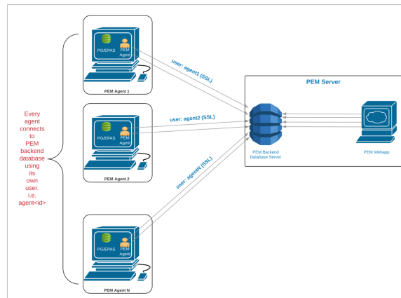
図 1 Connecting to the PEM database without pgBouncer
