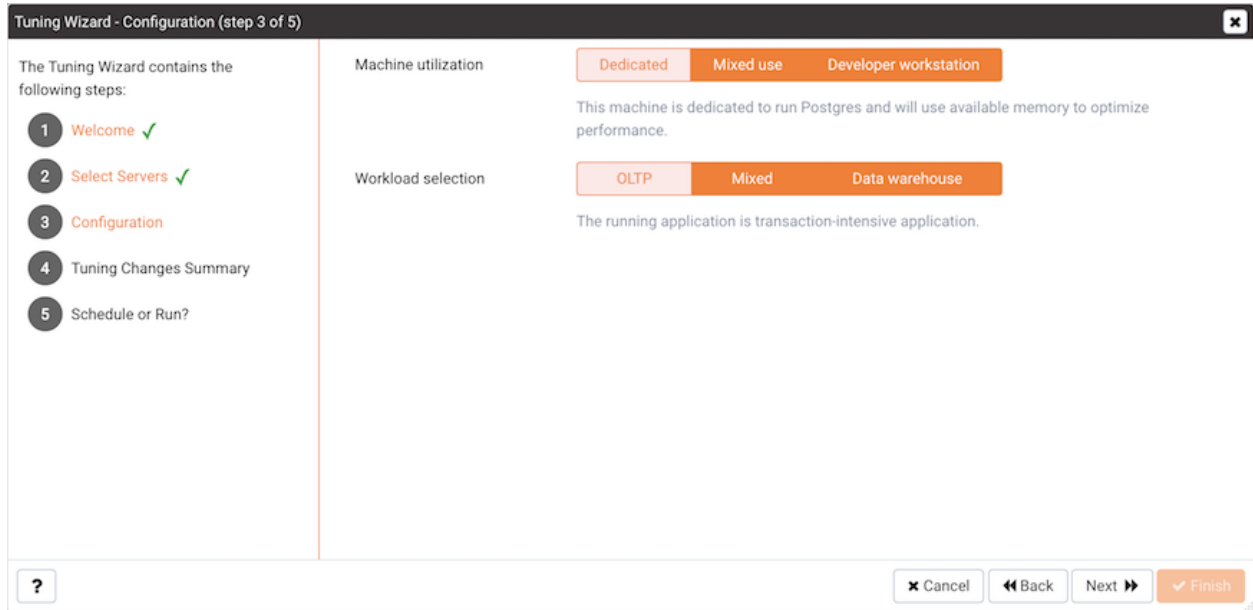
Fig. 3: The Configuration dialog
