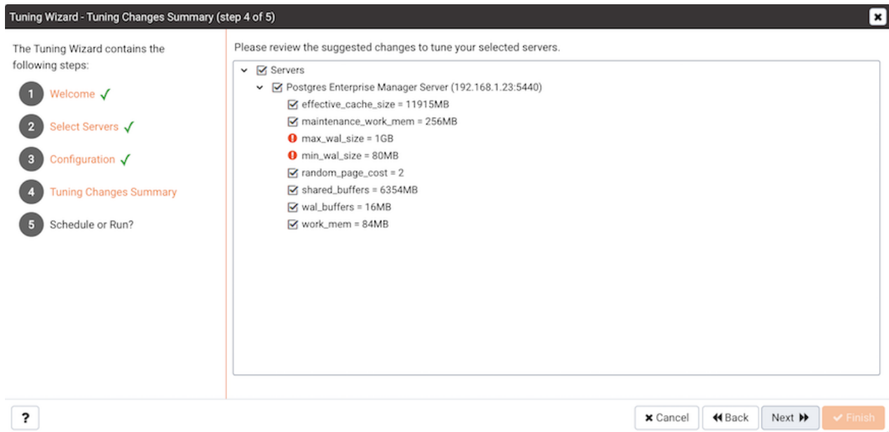
Fig. 4: The Tuning Changes Summary dialo
