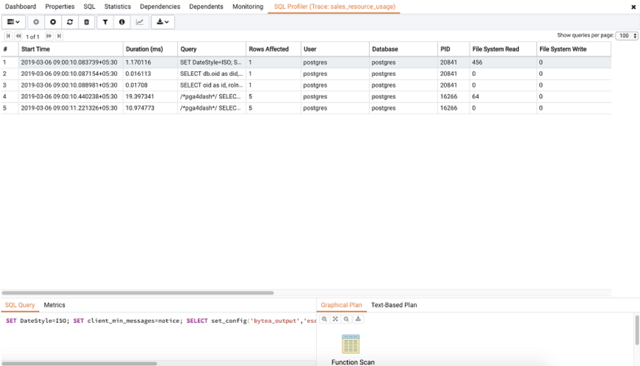
Fig. 4: The SQL Profiler tab, displaying the trace results
