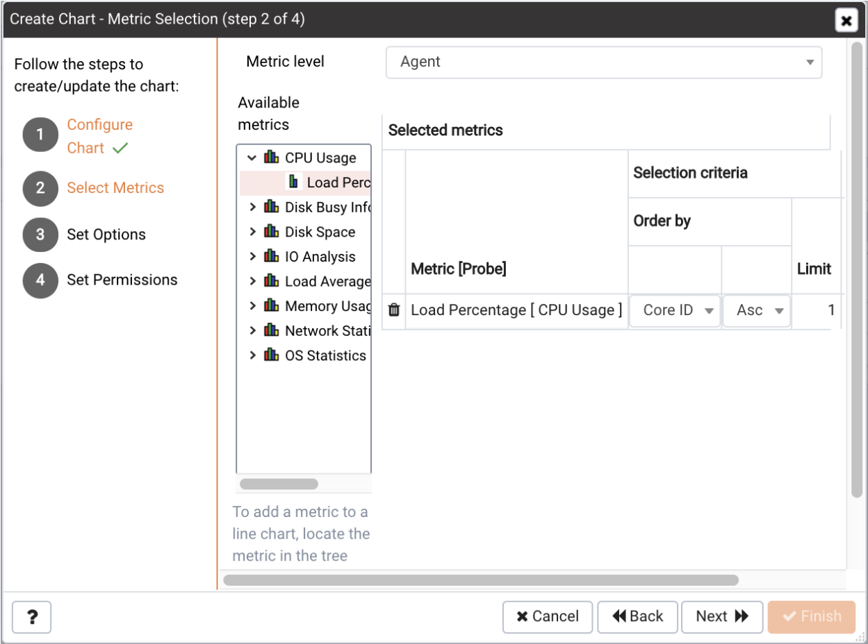
Fig. 12: Specifying the metrics that will be displayed
