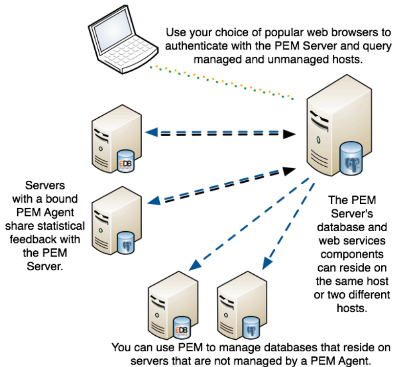
図 1 The Postgres Enterprise Manager general architecture
