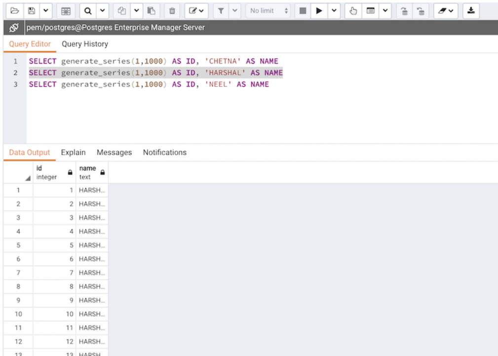
Fig. 5: Executing a command
