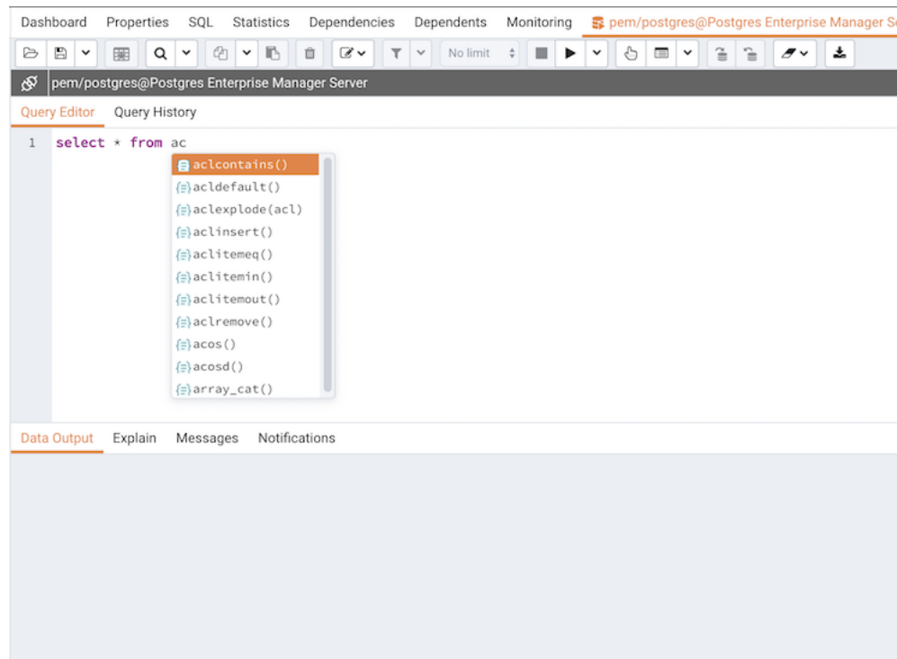
Fig. 4: Using Auto-complete
