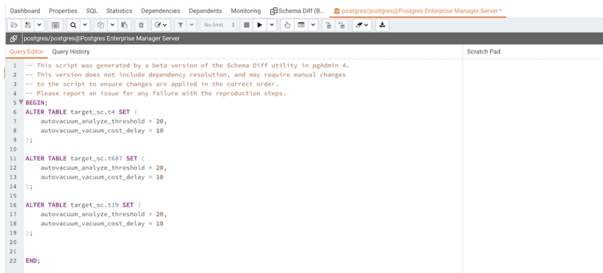
Fig. 7: Schema Diff dialog - Generate Script - Query Editor
