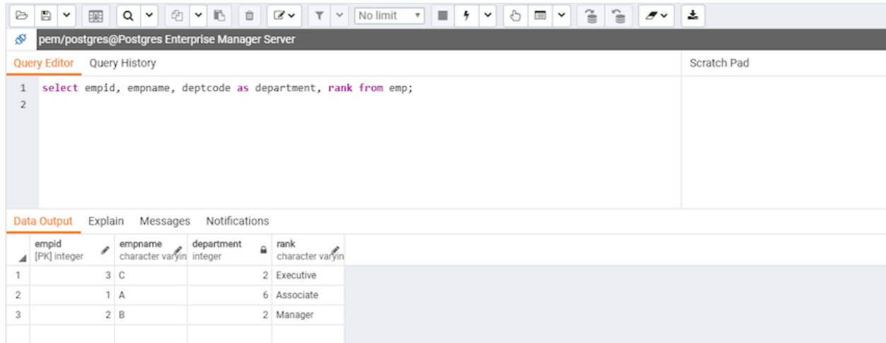
Fig. 8: Query Tool Editable Columns
