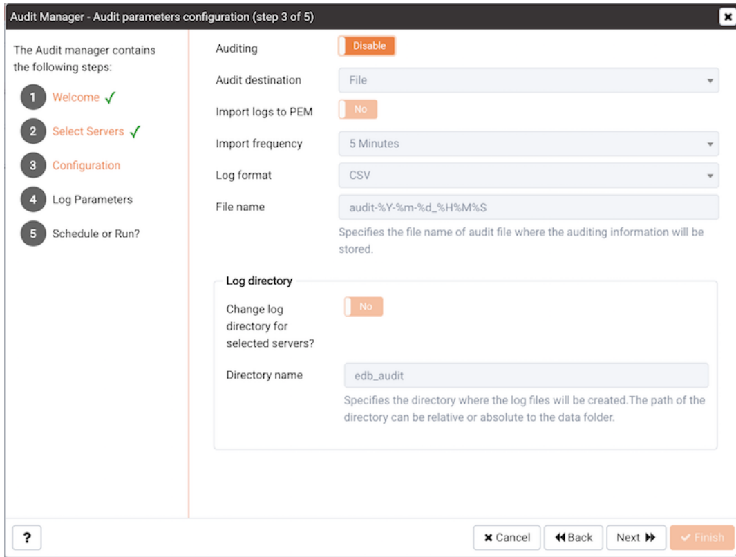
Fig. 5: The Auditing Parameters Configuration dialog
