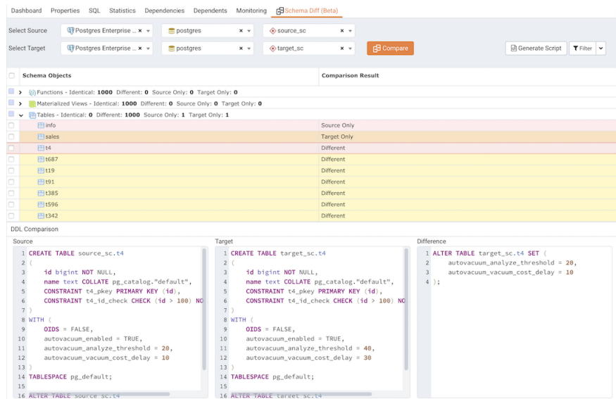
Fig. 5: Schema Diff dialog - DDL Comparison panel
