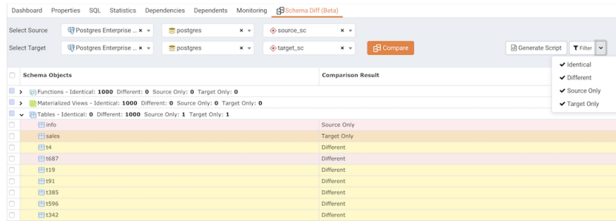
Fig. 4: Schema Diff dialog - Filter option
