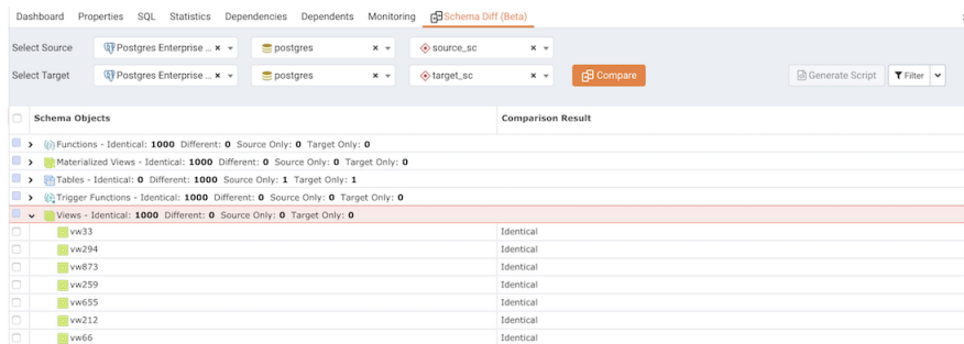
Fig. 3: Schema Diff dialog - Comparison Results
