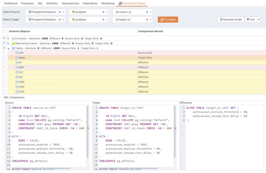
Fig. 1: Schema Diff dialog
