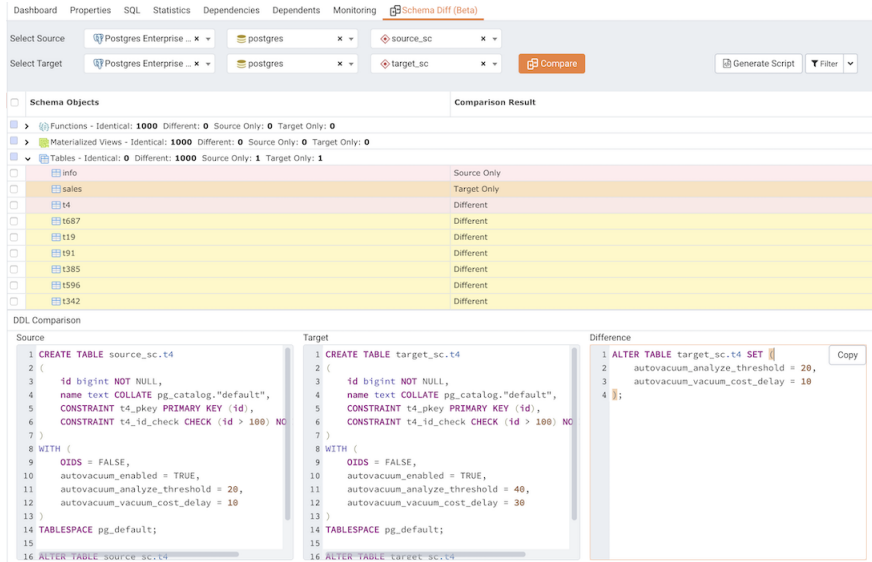
Fig. 6: Schema Diff dialog - Generate Script button
