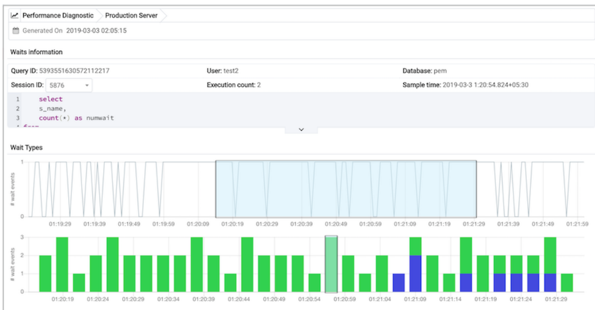
Fig. 7: The wait types bar graph
