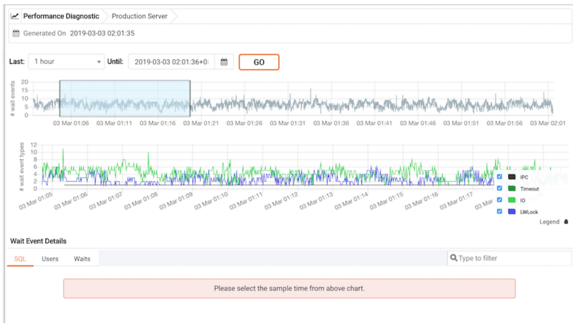
Fig. 4: Selecting a timeline
