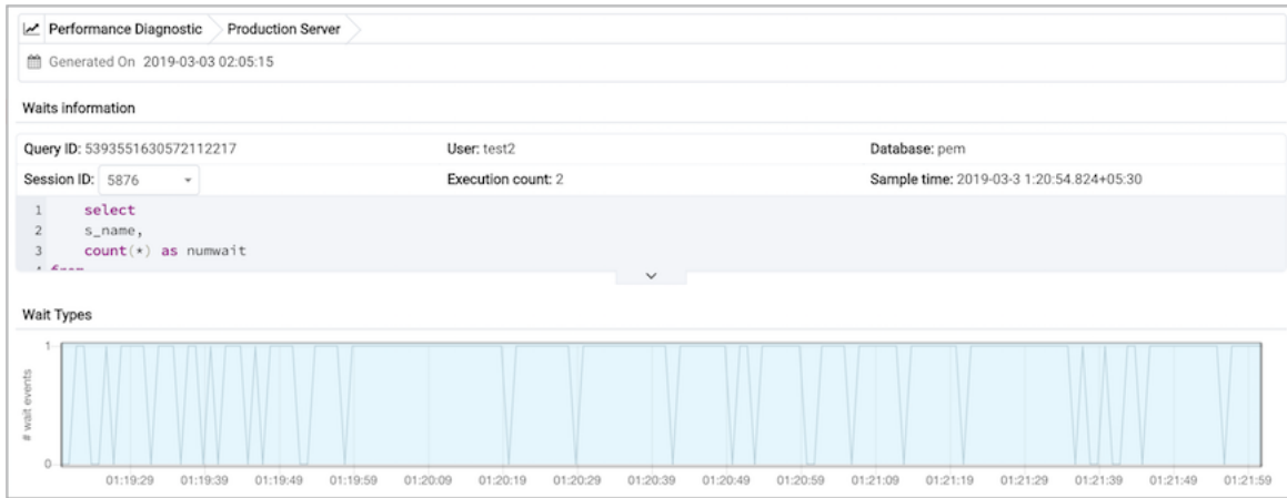
Fig. 6: The Waits information panel
