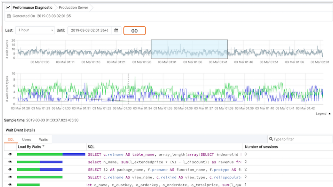
Fig. 5: Reviewing query details
