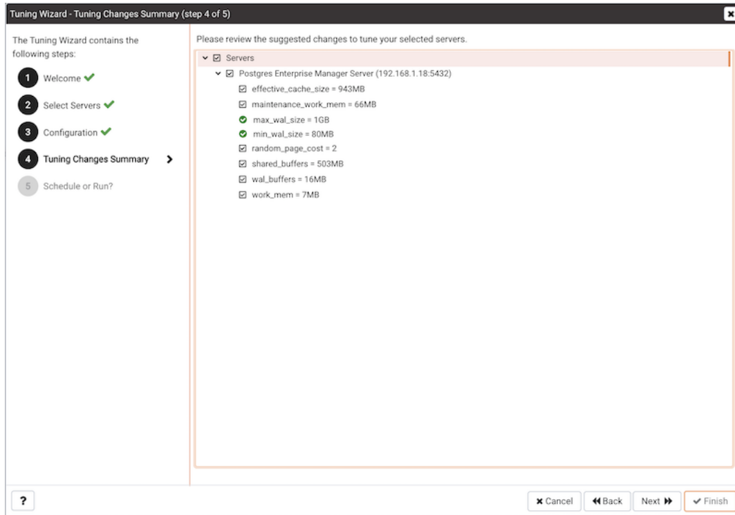
Fig. 4: The Tuning Changes Summary dialo
