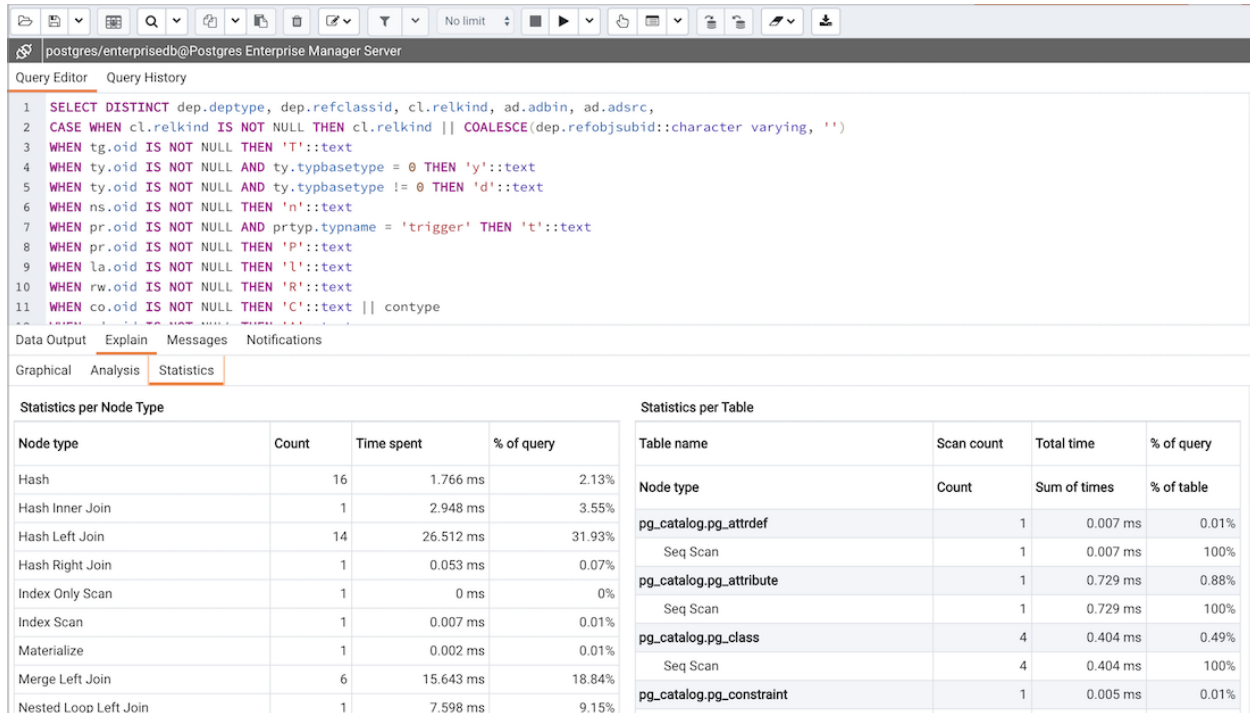
Fig. 12: Query Tool - Explain plan tab - Statistics tab
