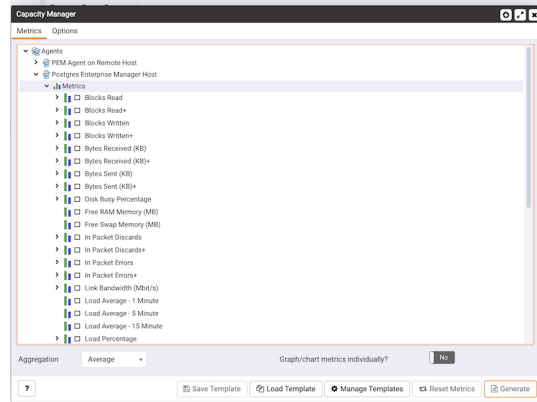
Fig. 2: Capacity Manager dialog - Metrics selection list
