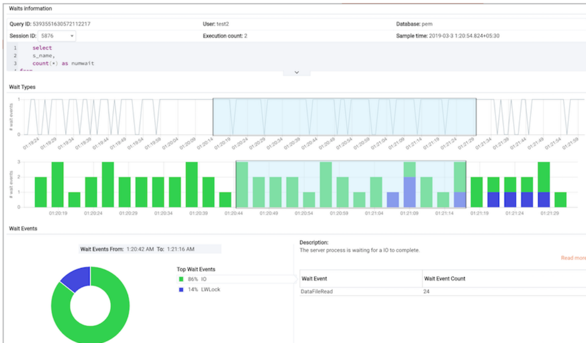
Fig. 8: The wait events donut chart
