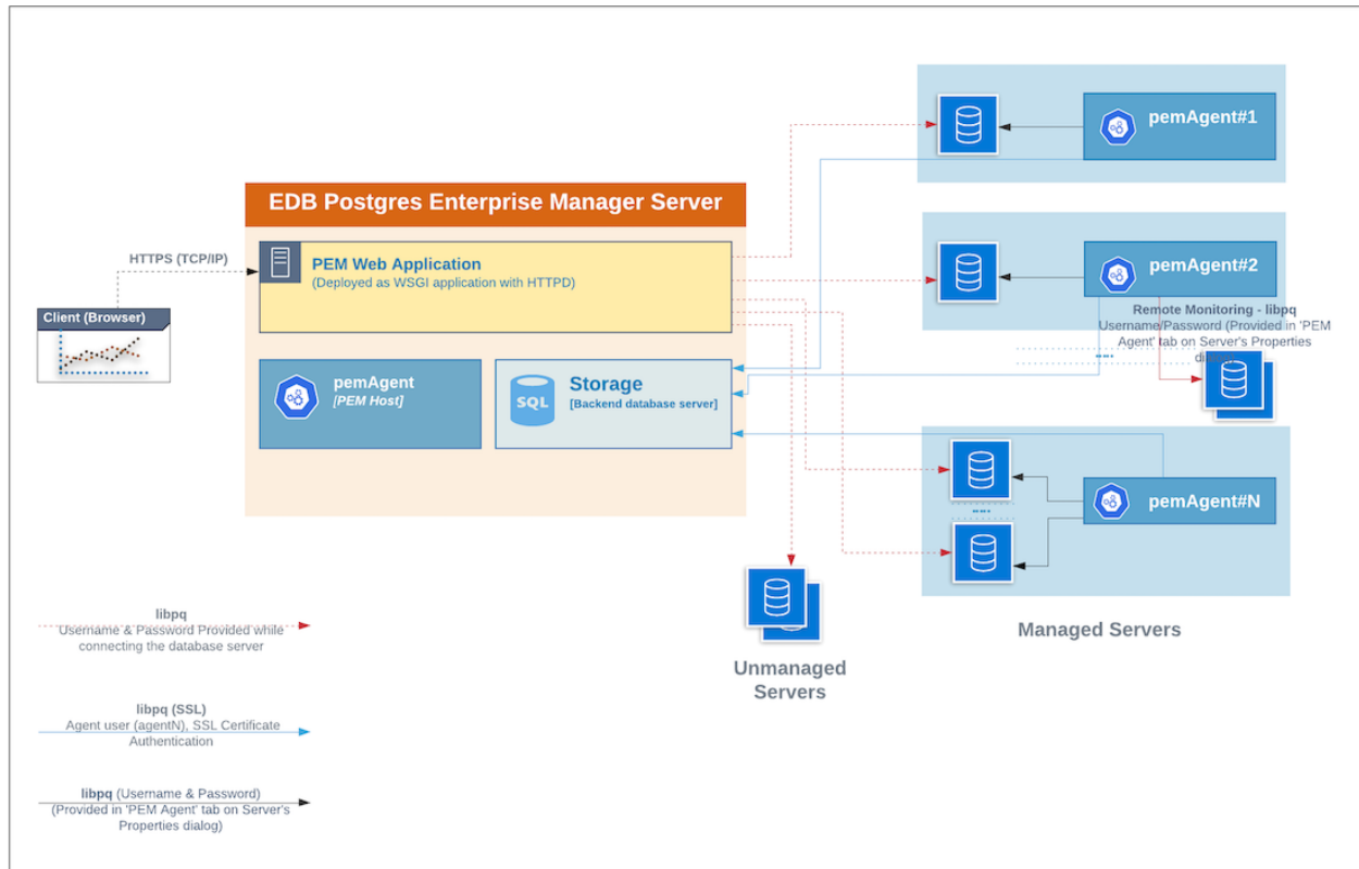
Fig. 1: A typical PEM installation.
