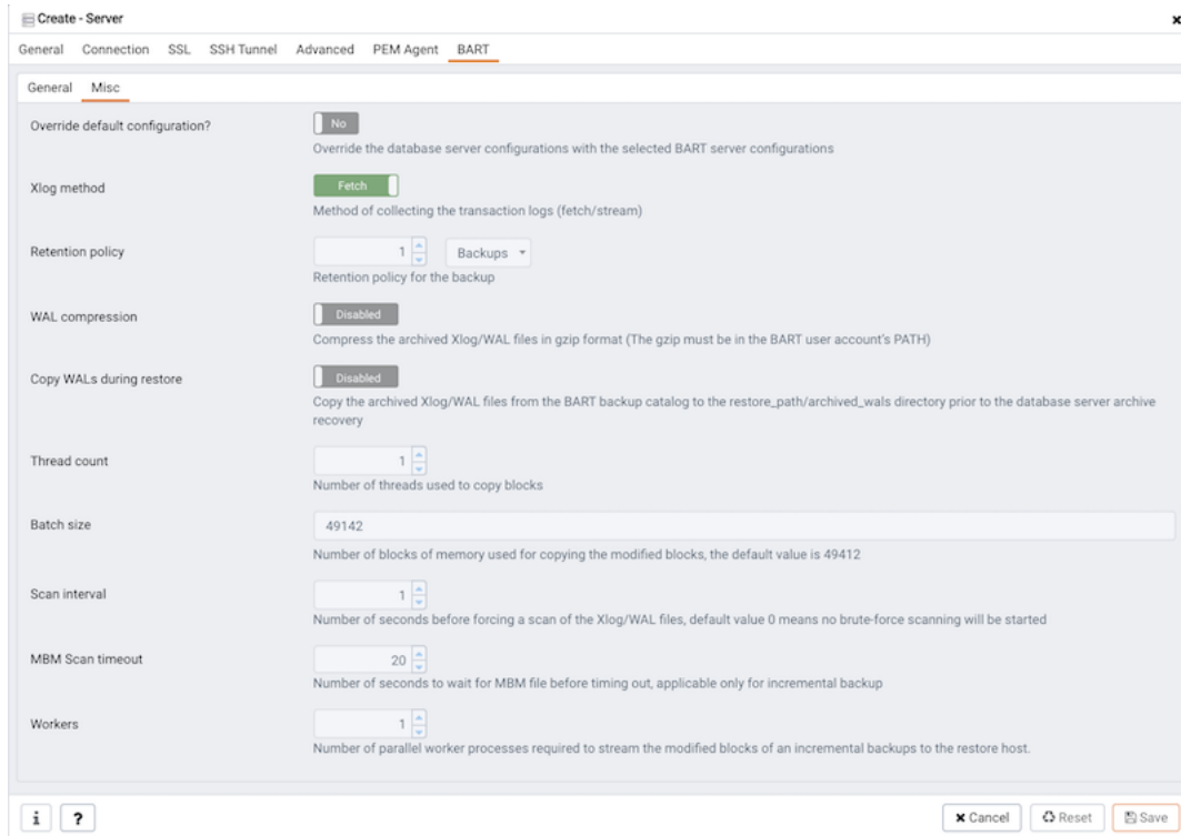
Fig. 4: The Create - Server dialog (BART - Misc tab)
