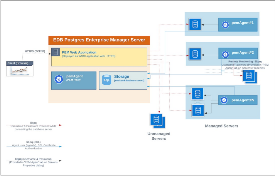
PEM Architecture
