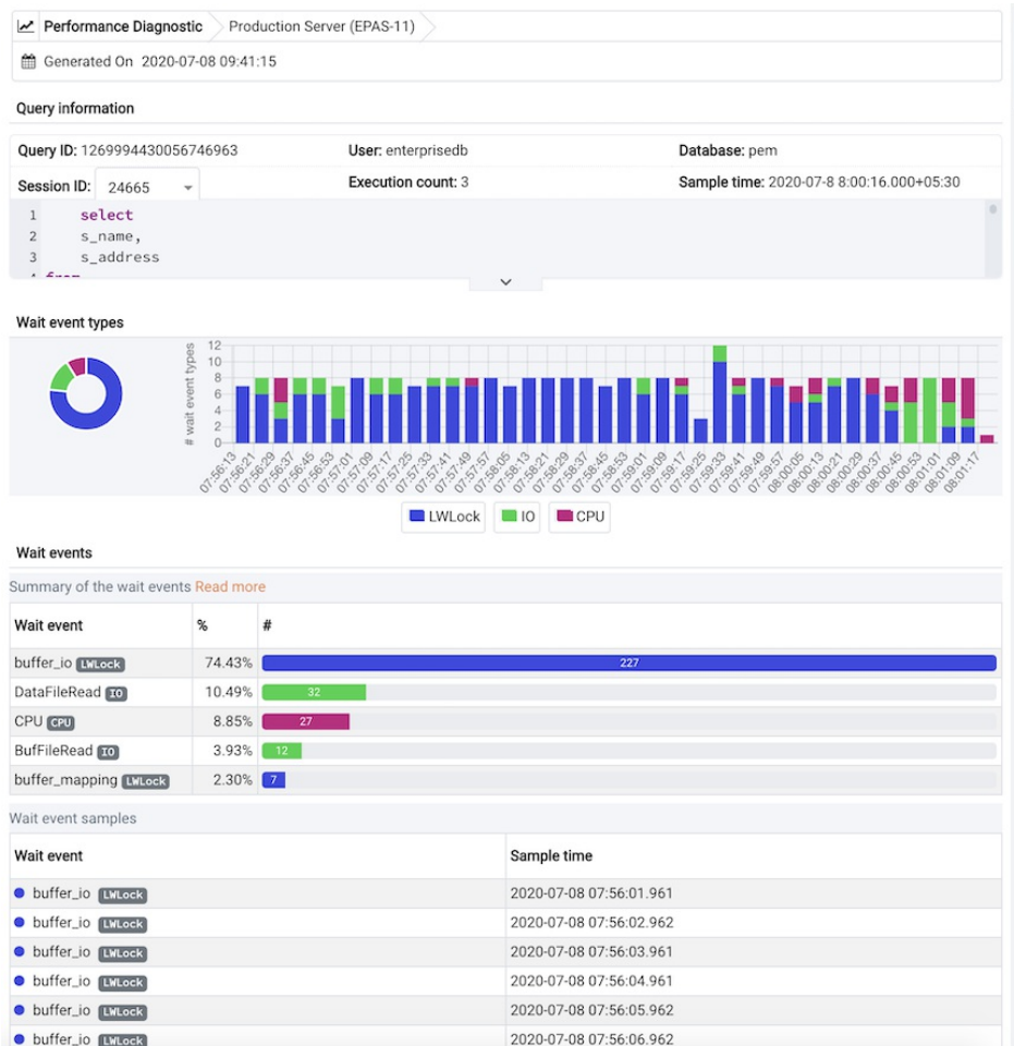
Performance Diagnostic - Query dashboard
