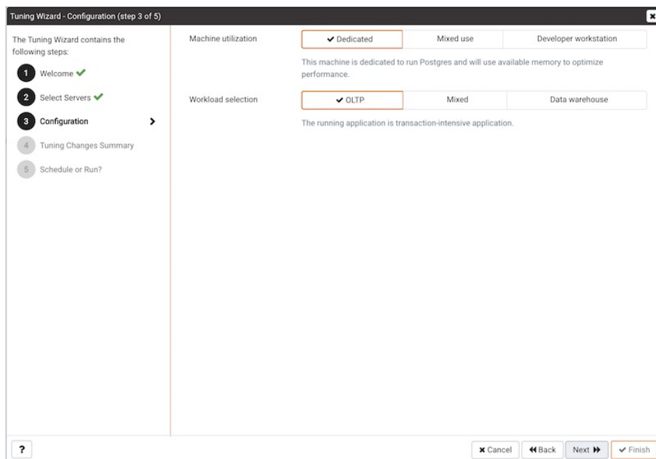
The Configuration dialog
