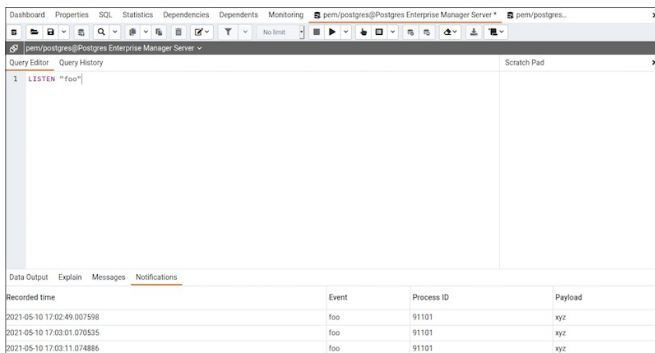
Query Tool - Output Notifications panel
