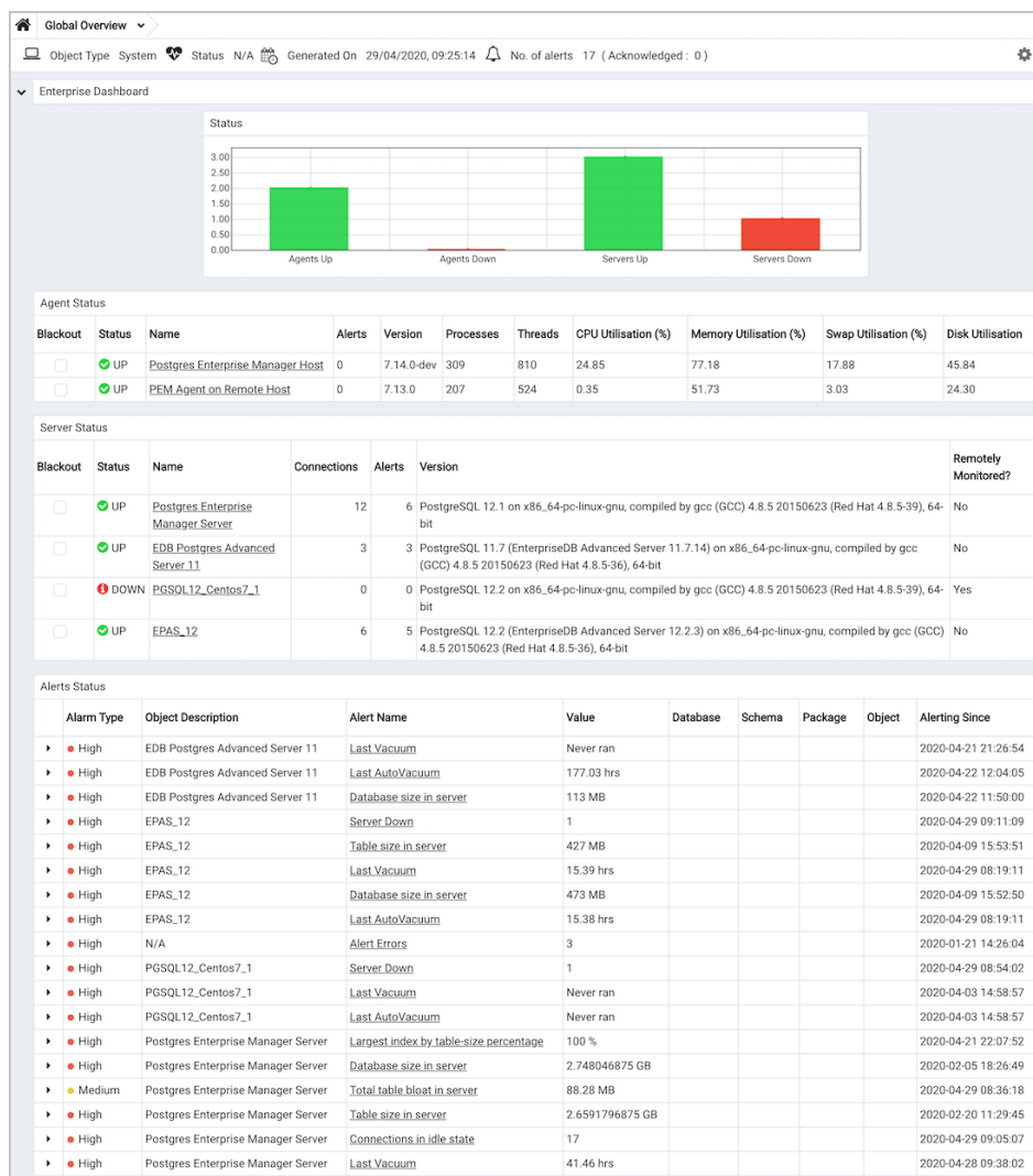
The Global Overview dashboard
