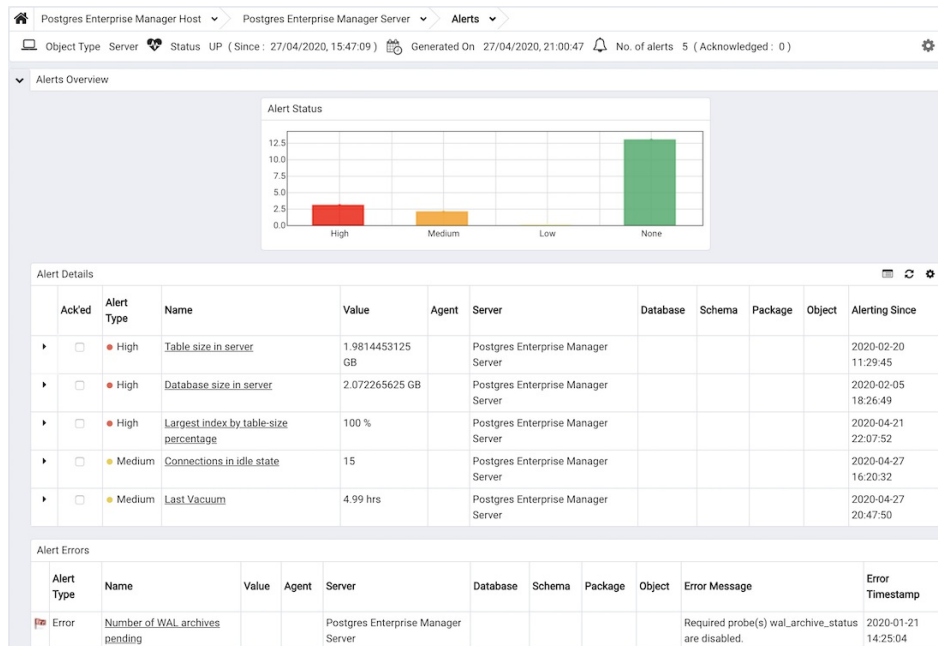
The Alerts Dashboard
