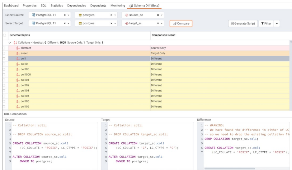
Schema Diff dialog
