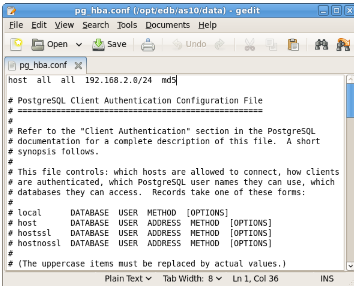
図 5 PEM entries in the pg_hba.conf file
