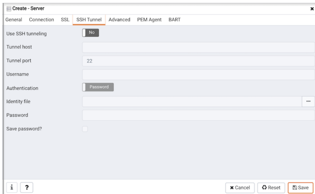
図 5 The SSH Tunnel tab of the Create – Server dialog
