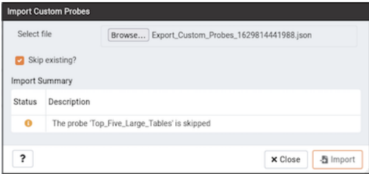
Fig. 29: Custom Probes - Import Skipped Message
