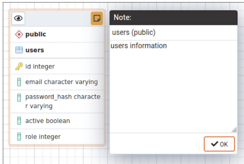
Fig. 8: ERD Tool - Table Notes
