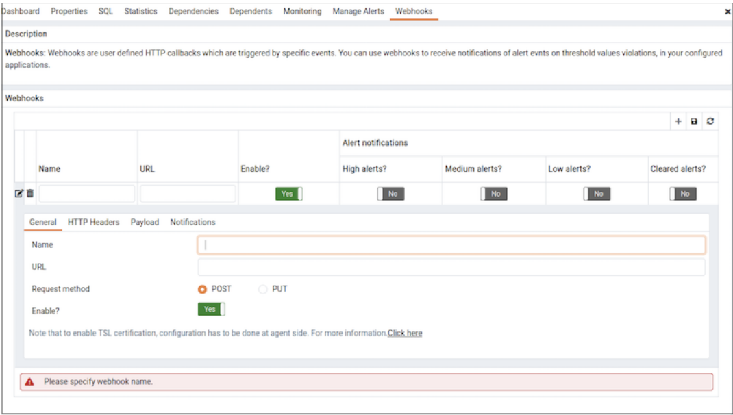
Fig. 70: Webhooks - Add New Webhook - General Tab
