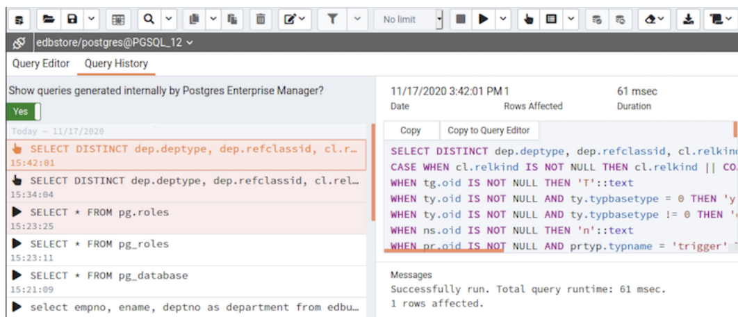
Fig. 18: Query Tool - Query History tab
