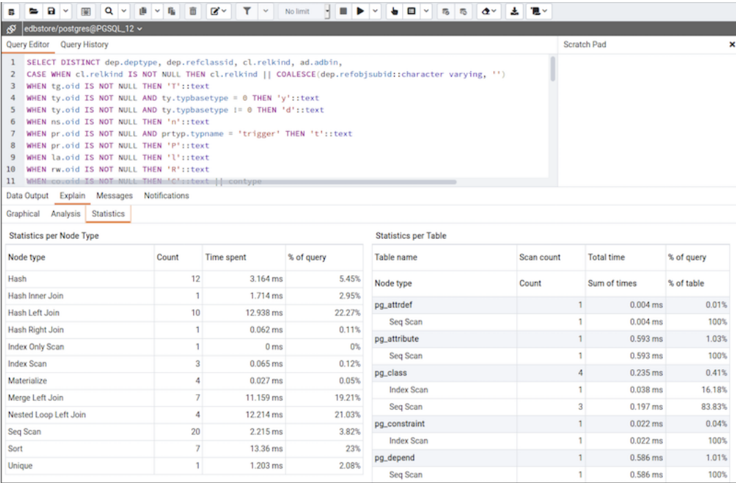
Fig. 12: Query Tool - Explain plan tab - Statistics tab
