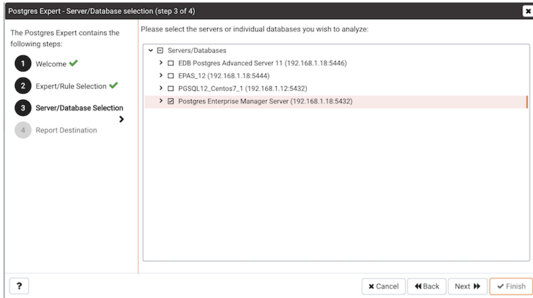
Fig. 3: The Servers/Databases dialog
