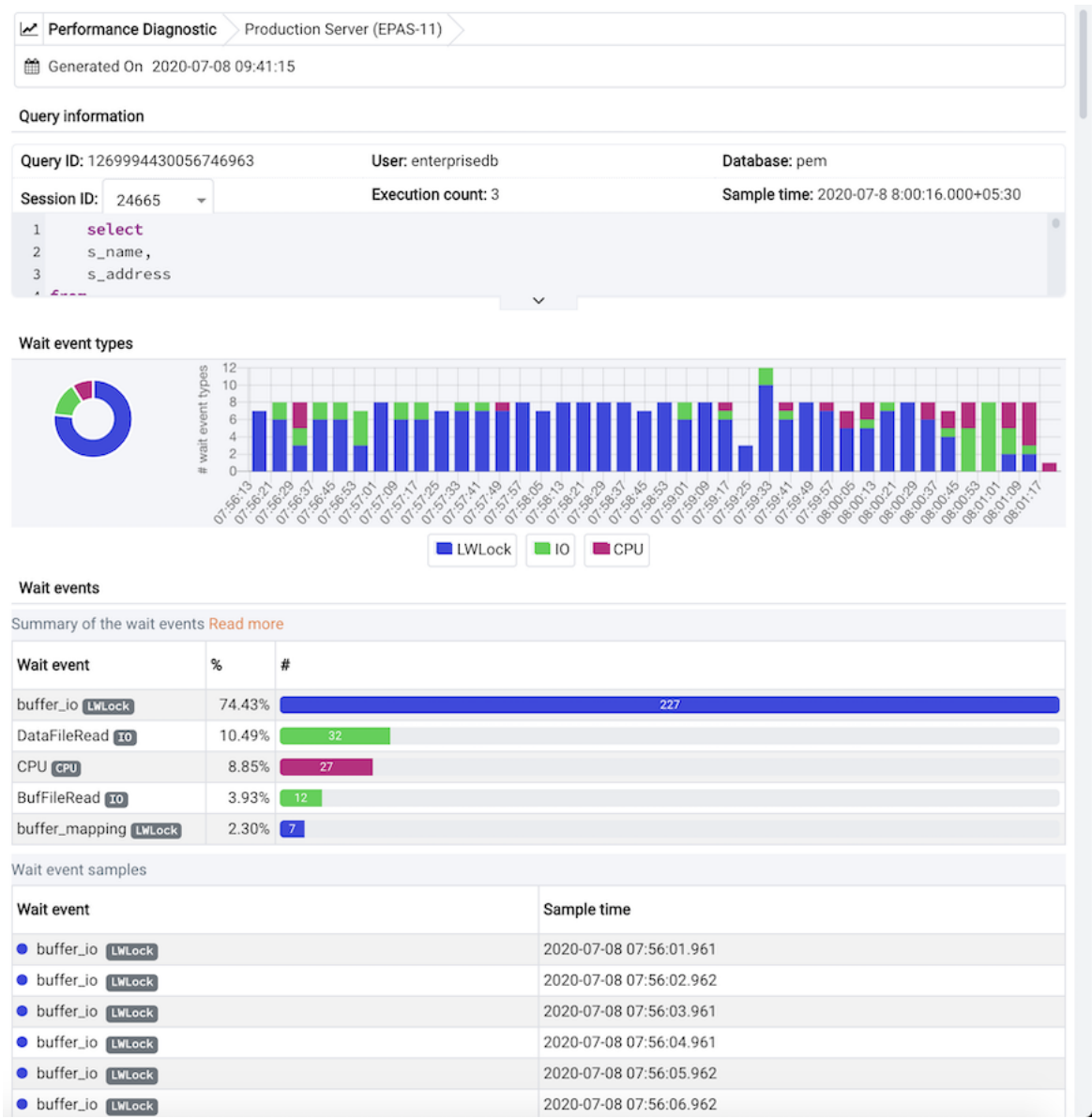
Fig. 7: Performance Diagnostic - Query dashboard
