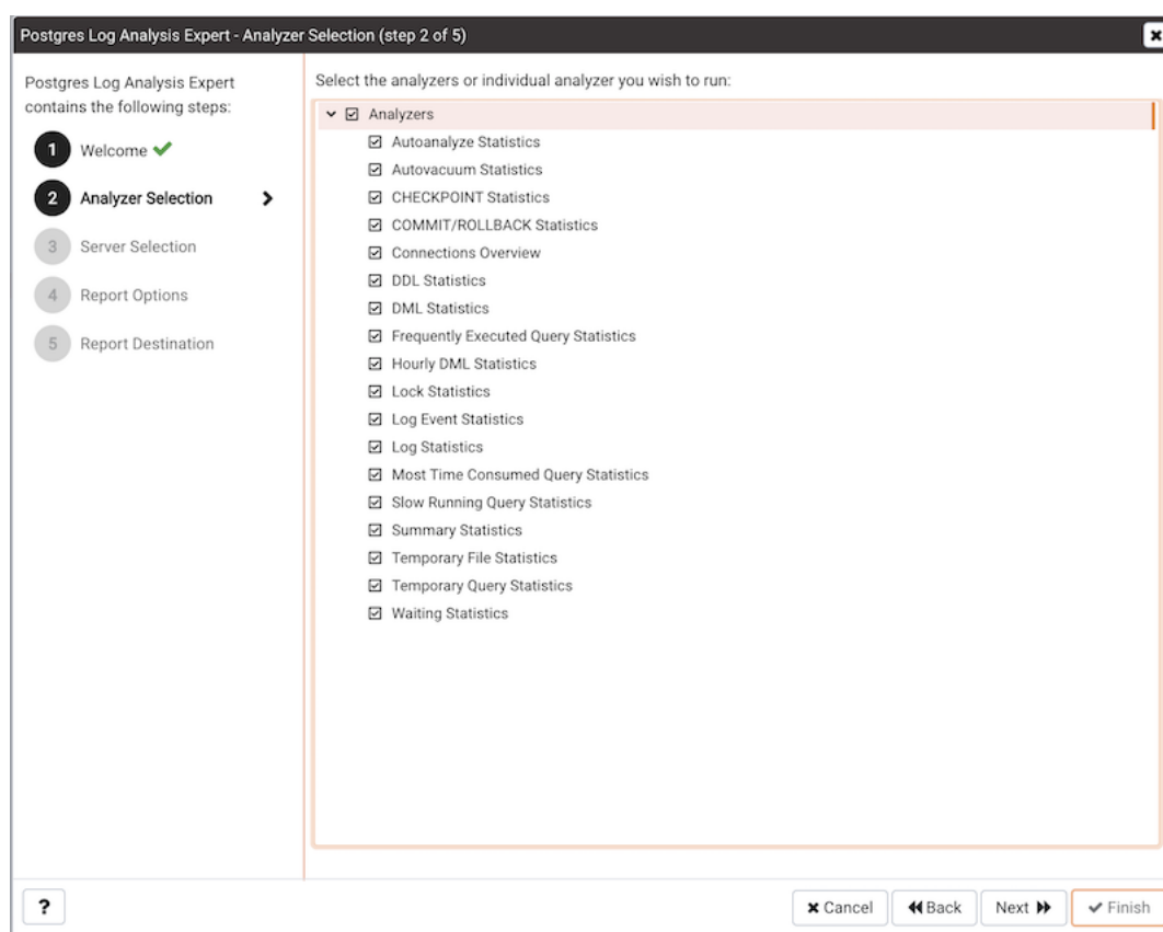
Fig. 11: The Analyzer selection dialog
