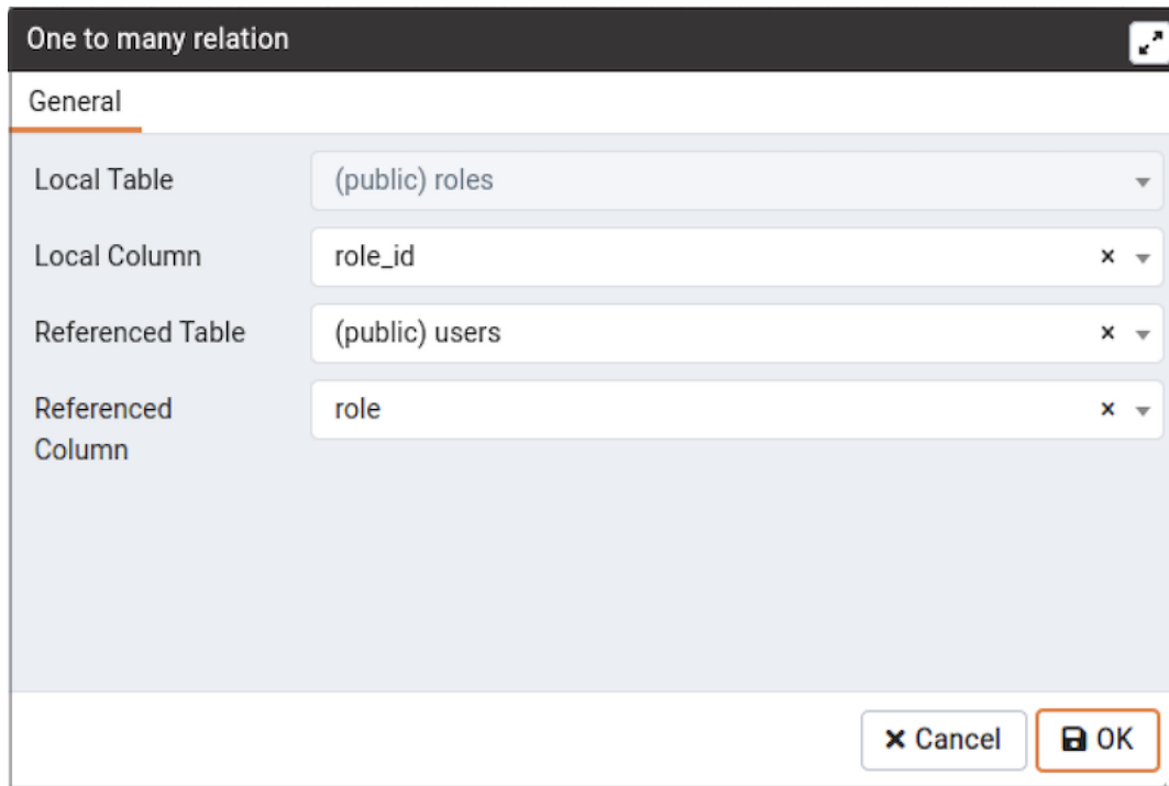
Fig. 5: ERD Tool - One to Many Dialog
