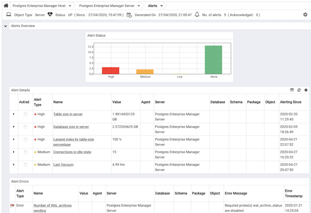
Fig. 36: The Alerts Dashboard
