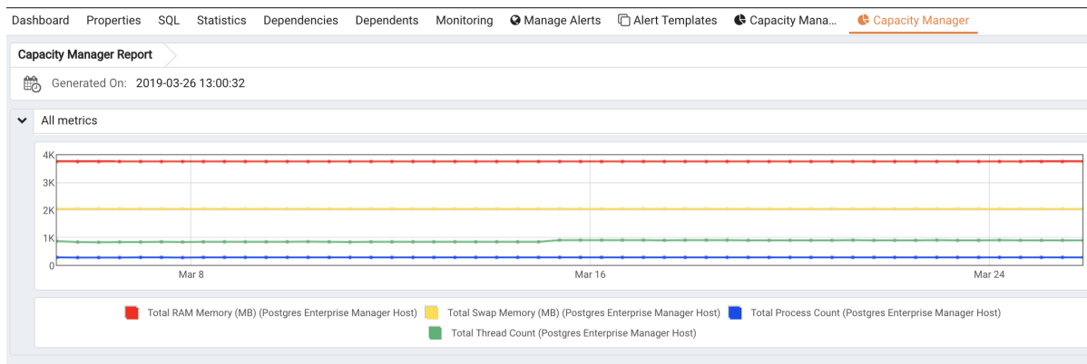
図 4: The Capacity Manager report
