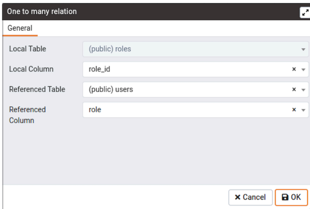
図 5: ERD Tool - One to Many Dialog
