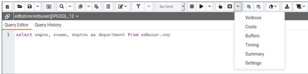
Figure 9: Query Tool - Toolbar Explain button
