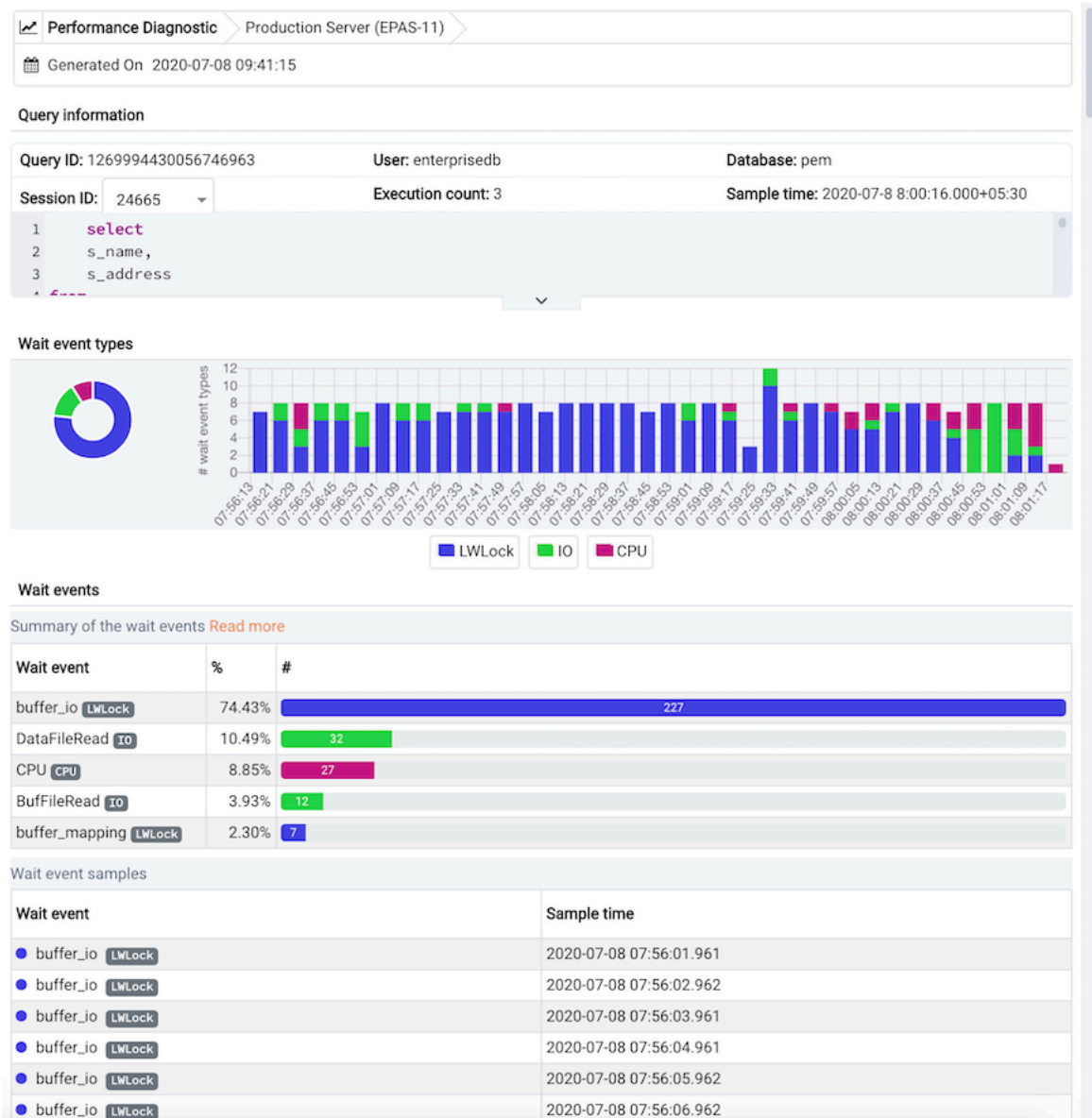
図 7: Performance Diagnostic - Query dashboard
