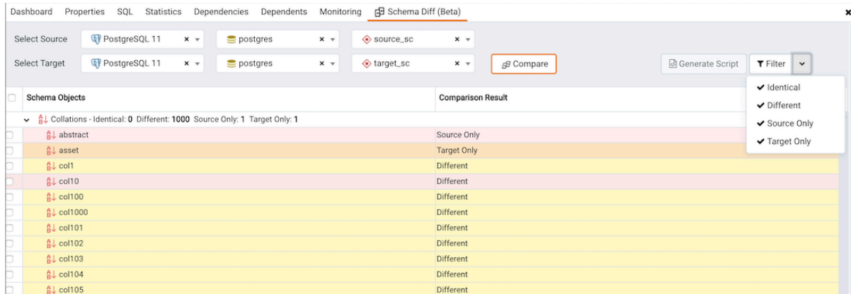
図 4: Schema Diff dialog - Filter option
