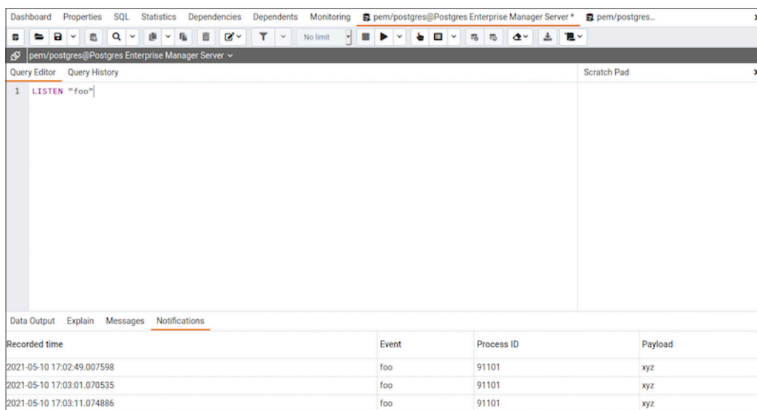
図 17: Query Tool - Output Notifications panel
