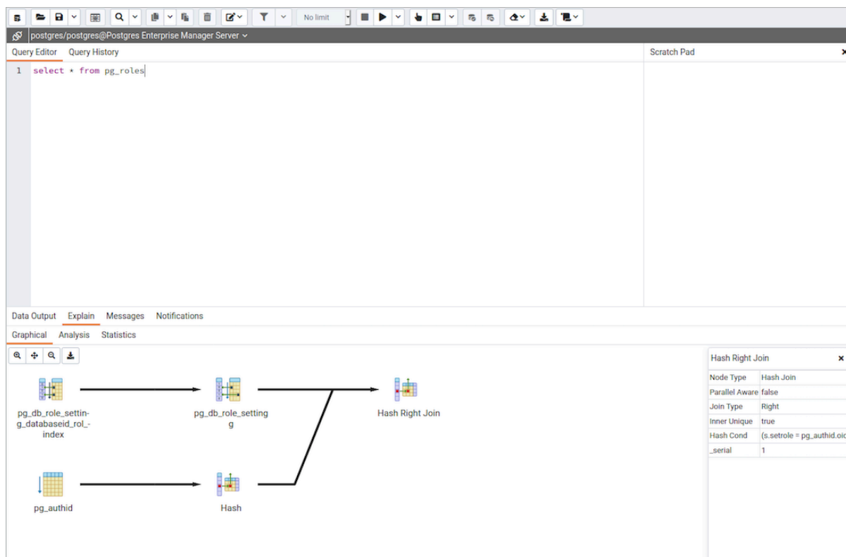
☒ 10: Query Tool - Explain tab - Graphical plan tab
