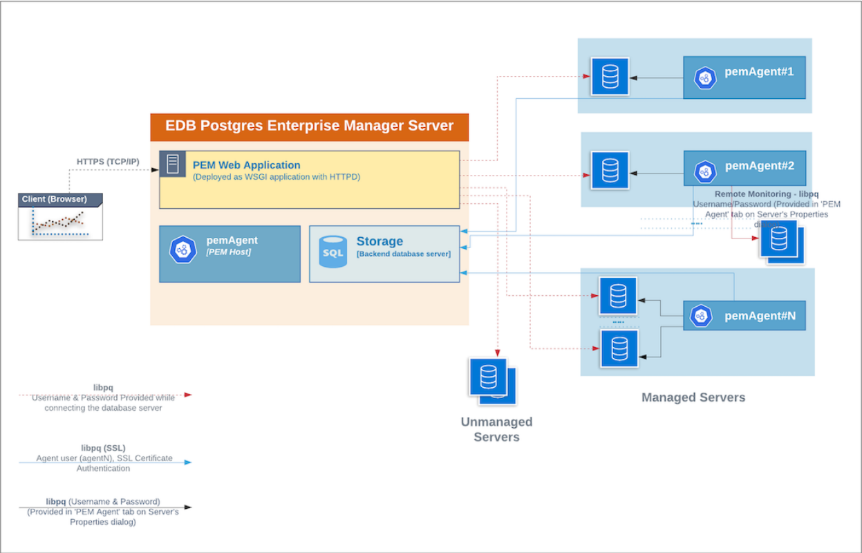
Fig. 1: PEM Architecture
