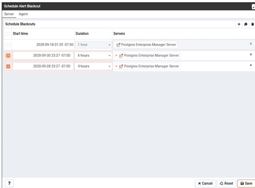
Fig. 65: Schedule Alert Blackout - Select servers
