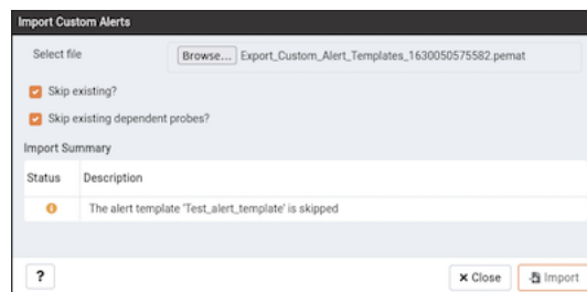
Fig. 48: Alert Templates Skip Both
