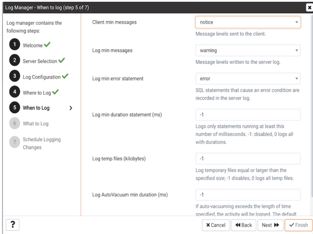
Fig. 5: The Log Manager When to Log dialog
