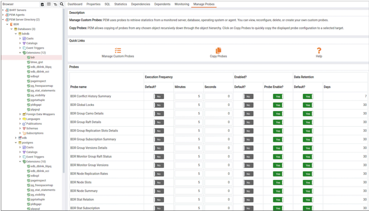
図 20: BDR Probes
