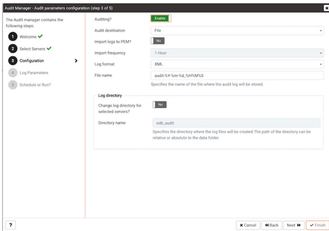
図 5: The Auditing Parameters Configuration dialog
