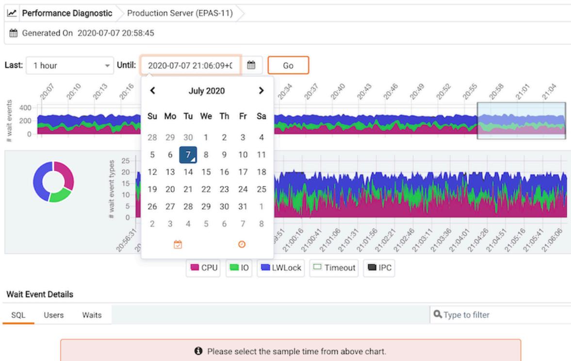
図 3: Performance Diagnostic dashboard - Time Changes option
