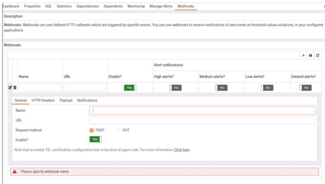
図 71: Webhooks - Add New Webhook - General Tab
