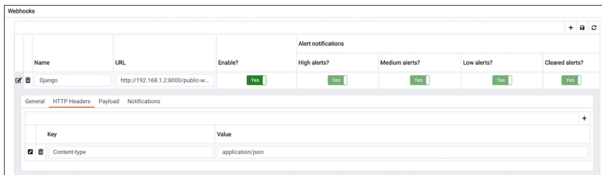
図 74: Webhooks - Add New Webhook - HTTP Headers Tab
