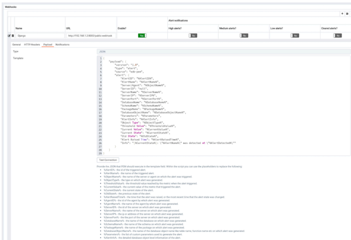
図 75: Webhooks - Add New Webhook - Payload Tab
