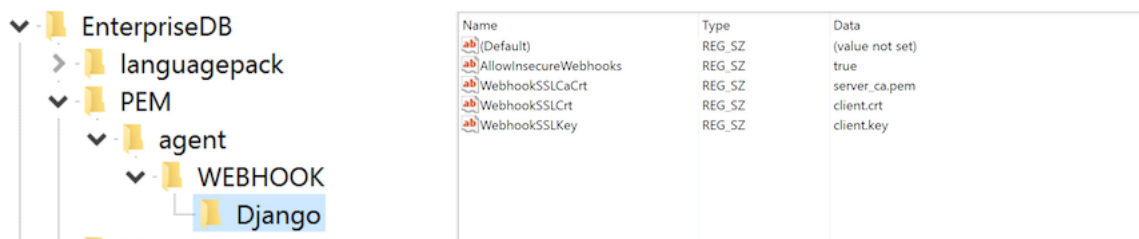
図 73: Example - Webhook SSL Parameters in windows registry
