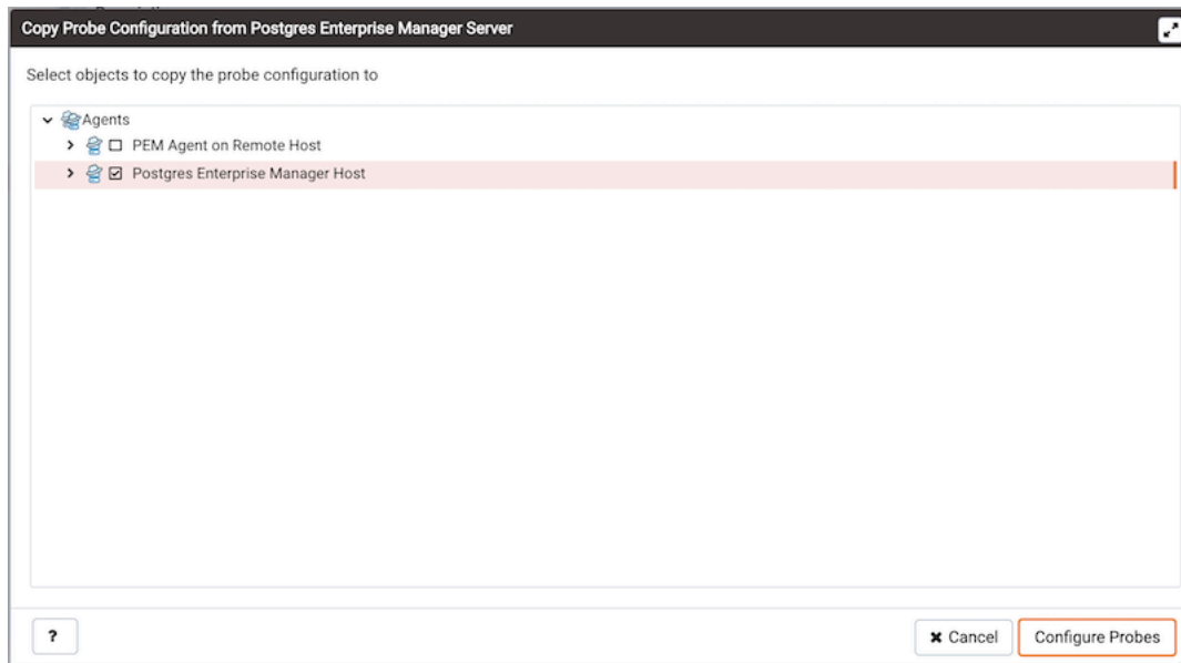
図 34: The Copy Probe Configuration tree control
