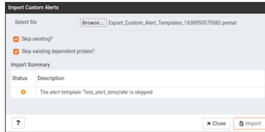
図 48: Alert Templates Skip Both
