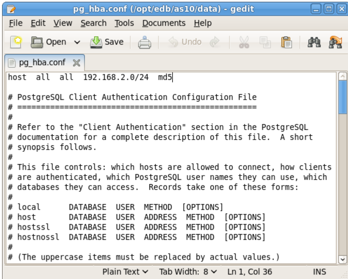
Fig. 2: PEM entries in the pg_hba.conf file
