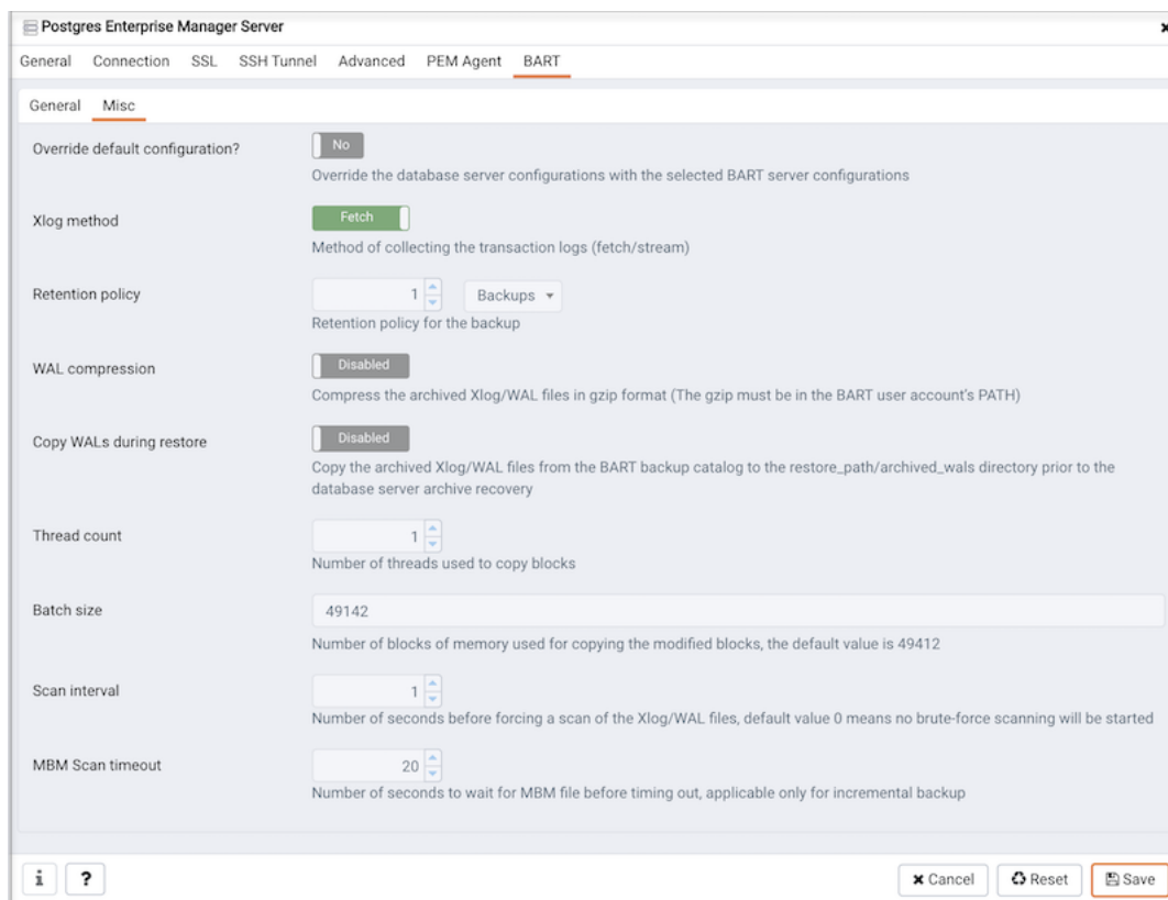
Fig. 10: The Create - Server dialog (BART - Misc tab)
