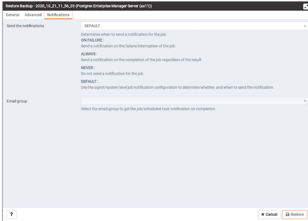
Fig. 12: The Restore Backup dialog - Notifications
