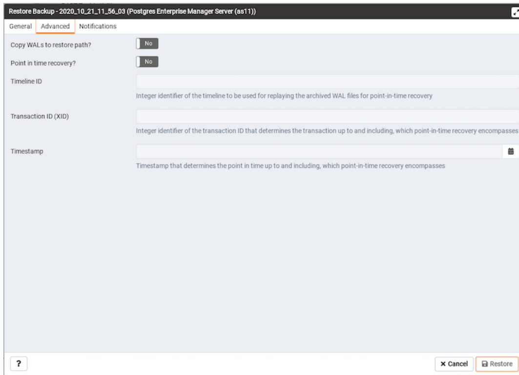
Fig. 11: The Restore Backup dialog - Advanced
