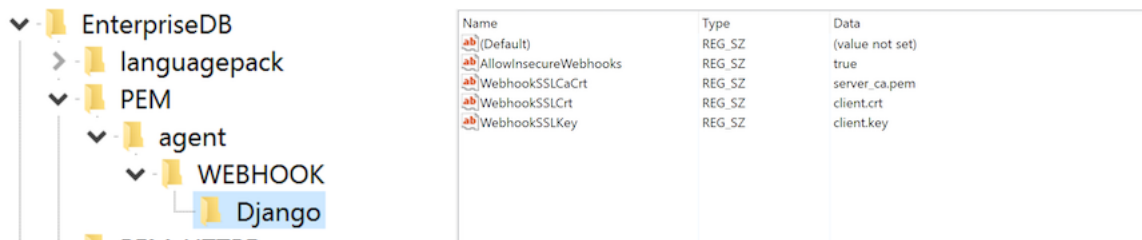
Fig. 51: Example - Webhook SSL Parameters in windows registry
