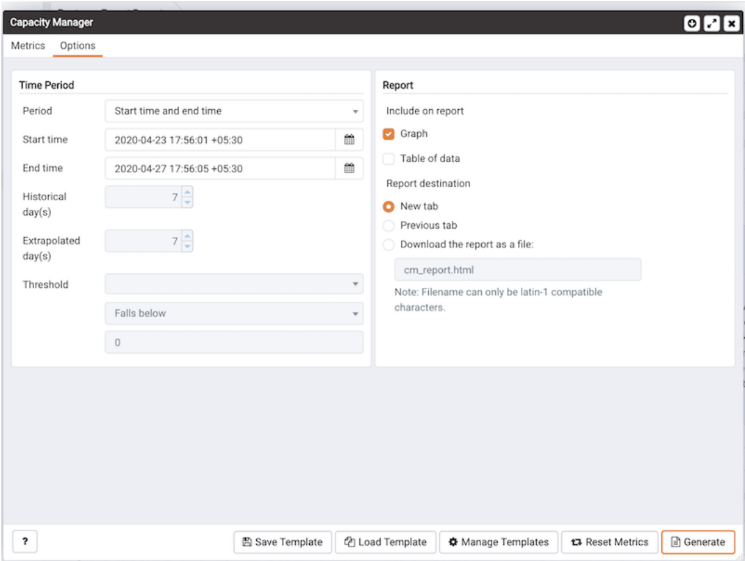
Fig. 3: Specify the time period, type, and destination of the report
