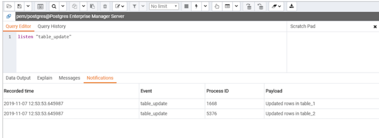
Fig. 15: Query Tool - Output Notifications tab
