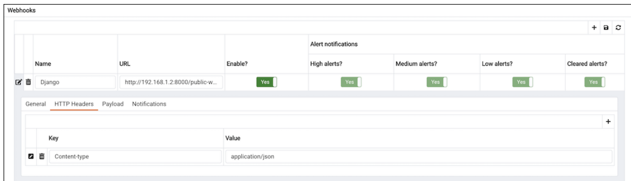
Fig. 52: Webhooks - Add New Webhook - HTTP Headers Tab
