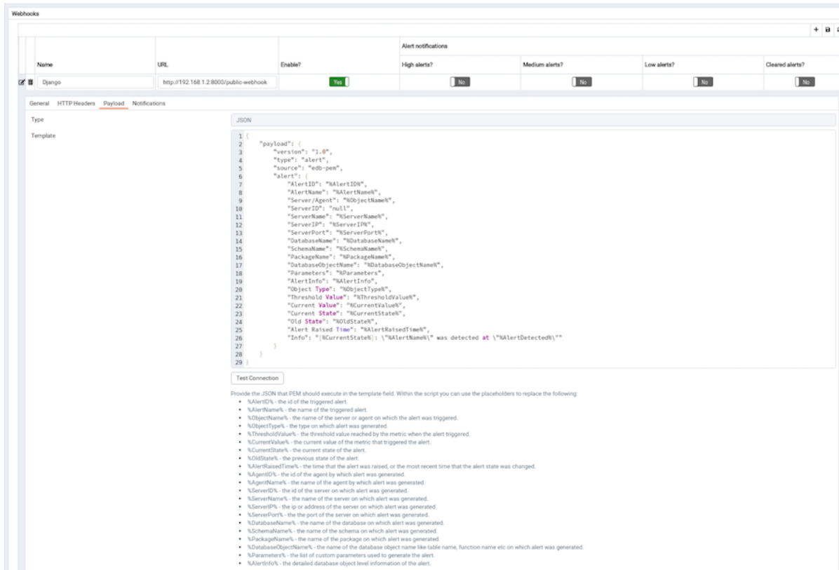
Fig. 53: Webhooks - Add New Webhook - Payload Tab
