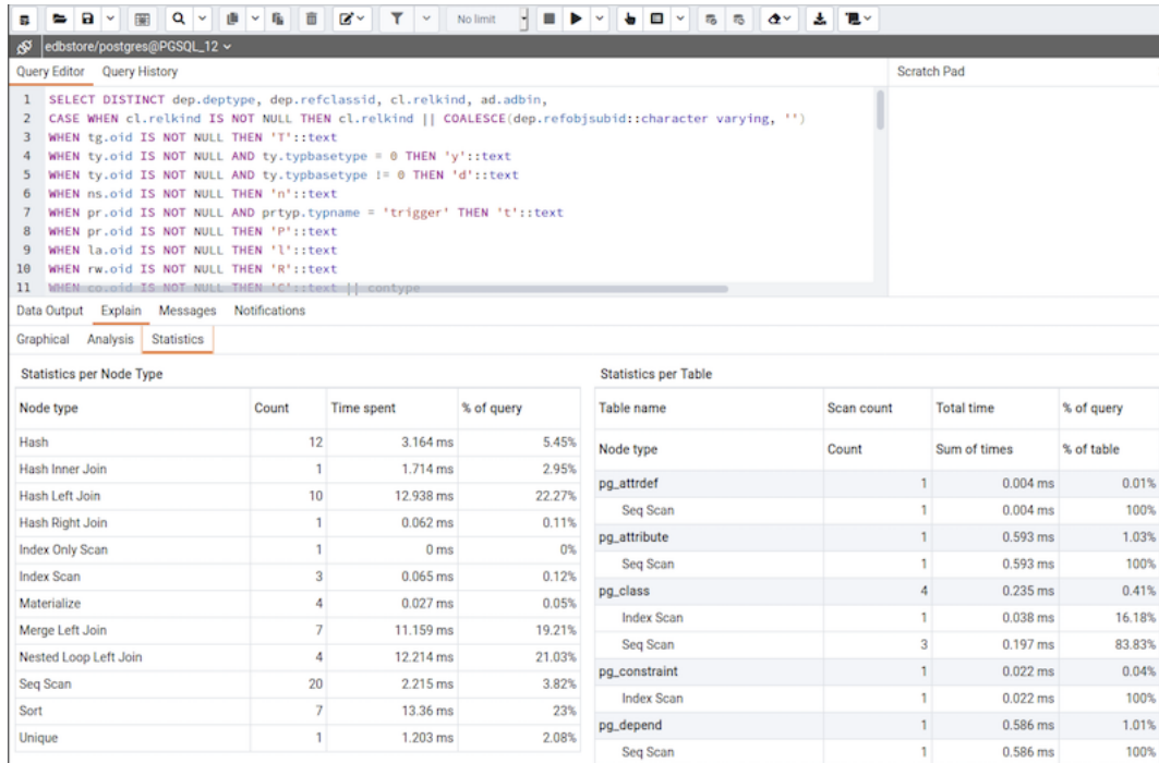
Fig. 12: Query Tool - Explain plan tab - Statistics tab
