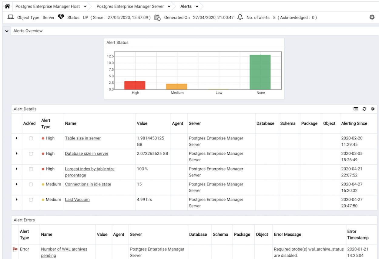
Fig. 30: The Alerts Dashboard
